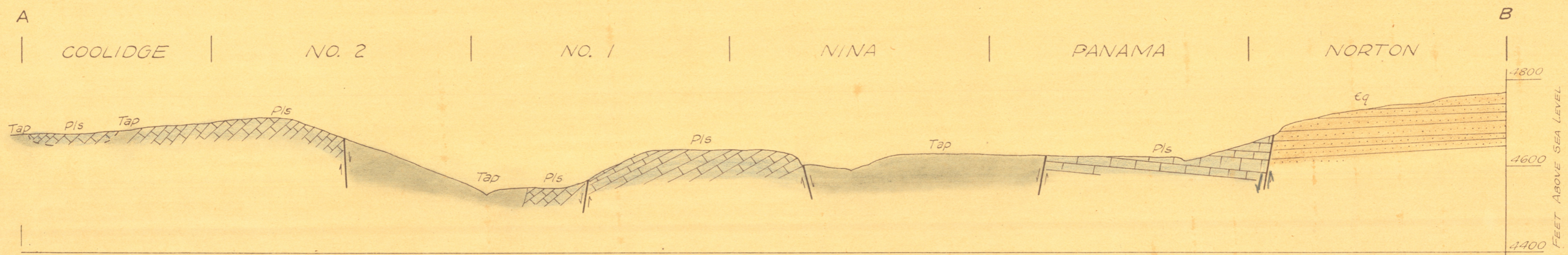
PLATE III CROSS SECTION ALONG LINE A-B OF PLATE II
