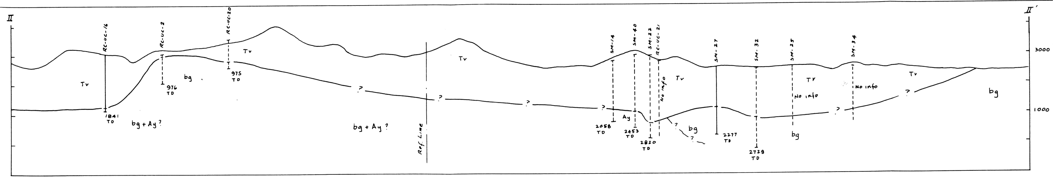
SECTION II-II'
