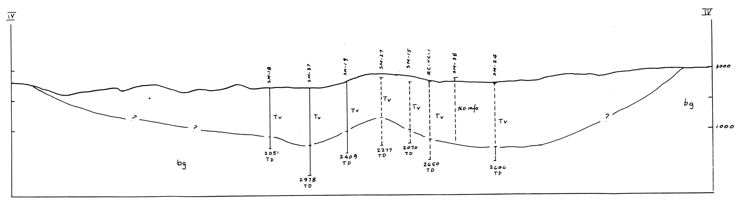
SECTION IV-IV'
