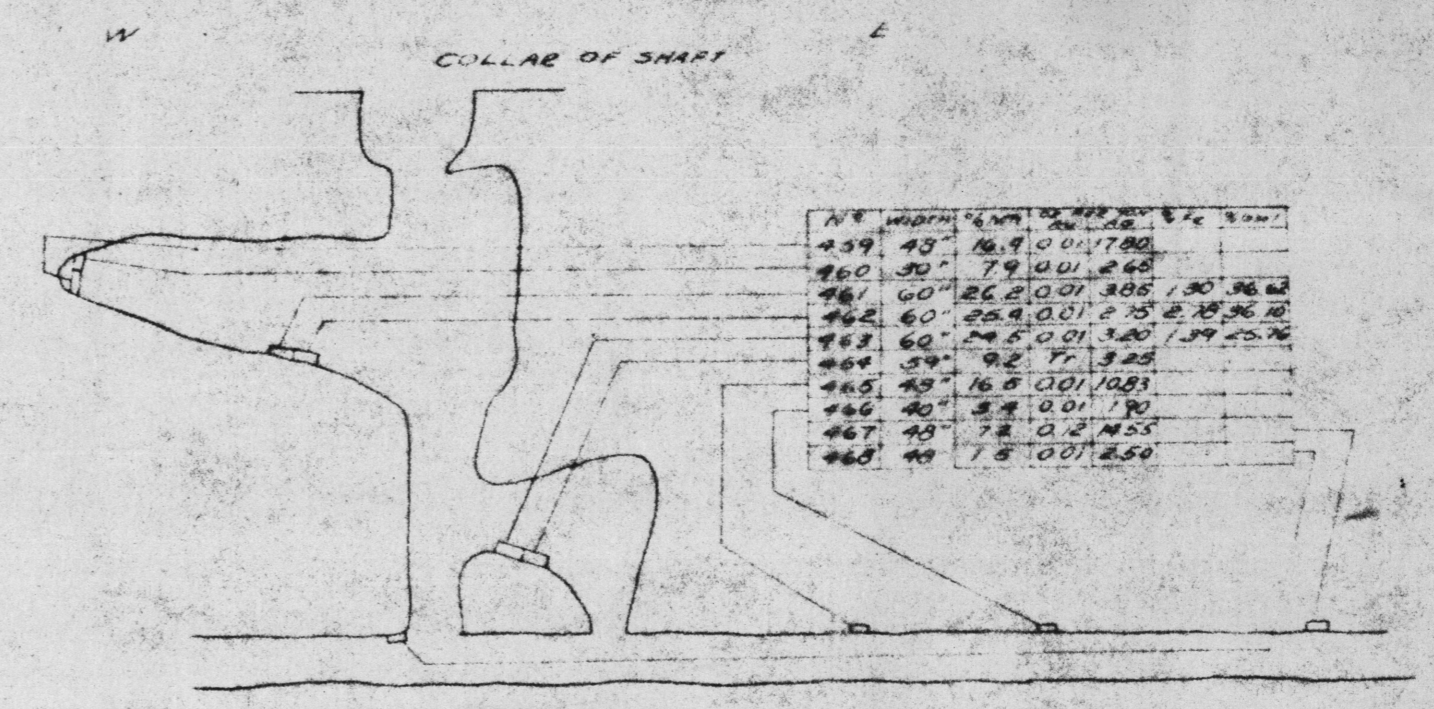
SECTION A-A' RATTLESNAKE SHAFT SCALE 1" = 40'
