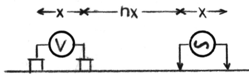
ELECTRODE CONFIGURATION
