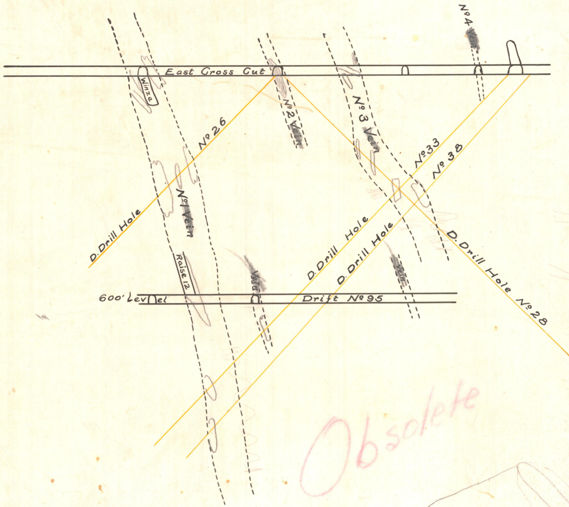
VERTICAL CROSS SECTION ON LINE OF D. Drill Hole EAST CROSS CUT 928 DRIFT No 95 TO SHOW THE RELATION OF ORE LENSES IN VEINS Nos 1, 2 928 3
