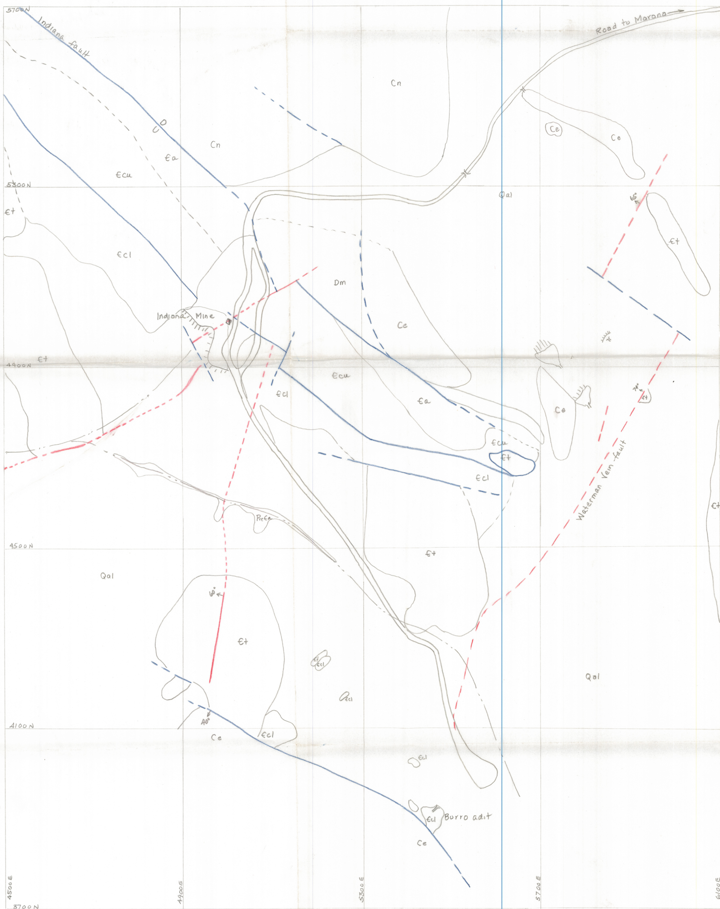
GEOLOGIC MAP OF INDIANA MINE AREA PIMA COUNTY, ARIZONA SCALE: 1" = 100'
