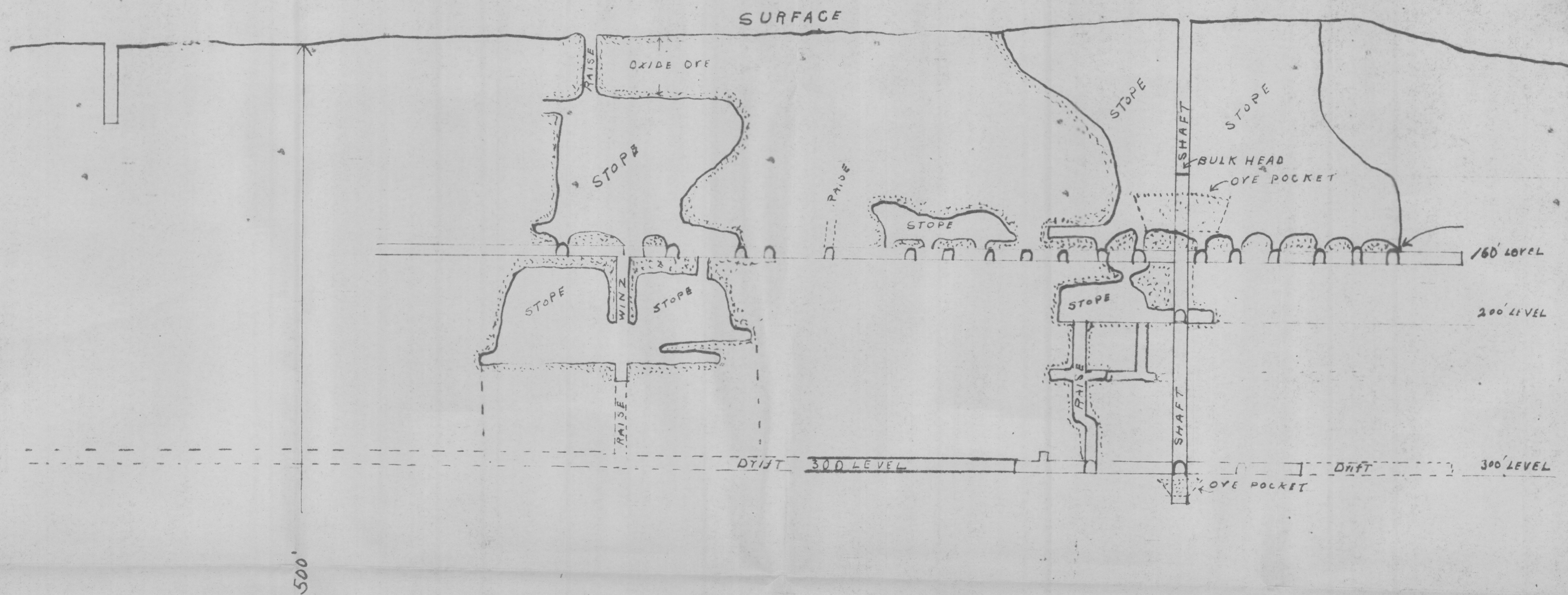
LONGITUDINAL SECTION SUMMIT MINE SCALE 1" = 50' SEP 20 1946
