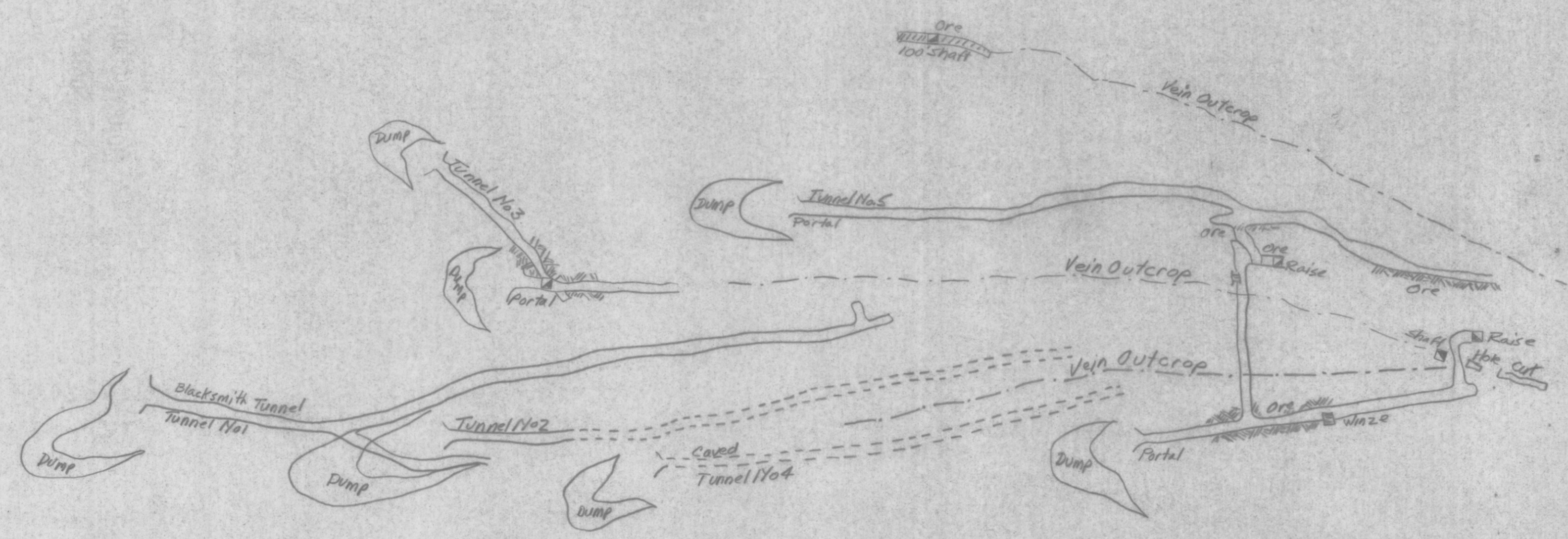
MAP OF A PORTION OF UNDERGROUND WORKS OF ST. LOUIS CLAIM MOHAVE COUNTY ARIZONA COMPILED FROM SURVEYS AND OTHER SOURCES TO ACCOMPANY REPORT OF R.E. JACOBSON. SCALE 1"=60' JAN. 1922.
