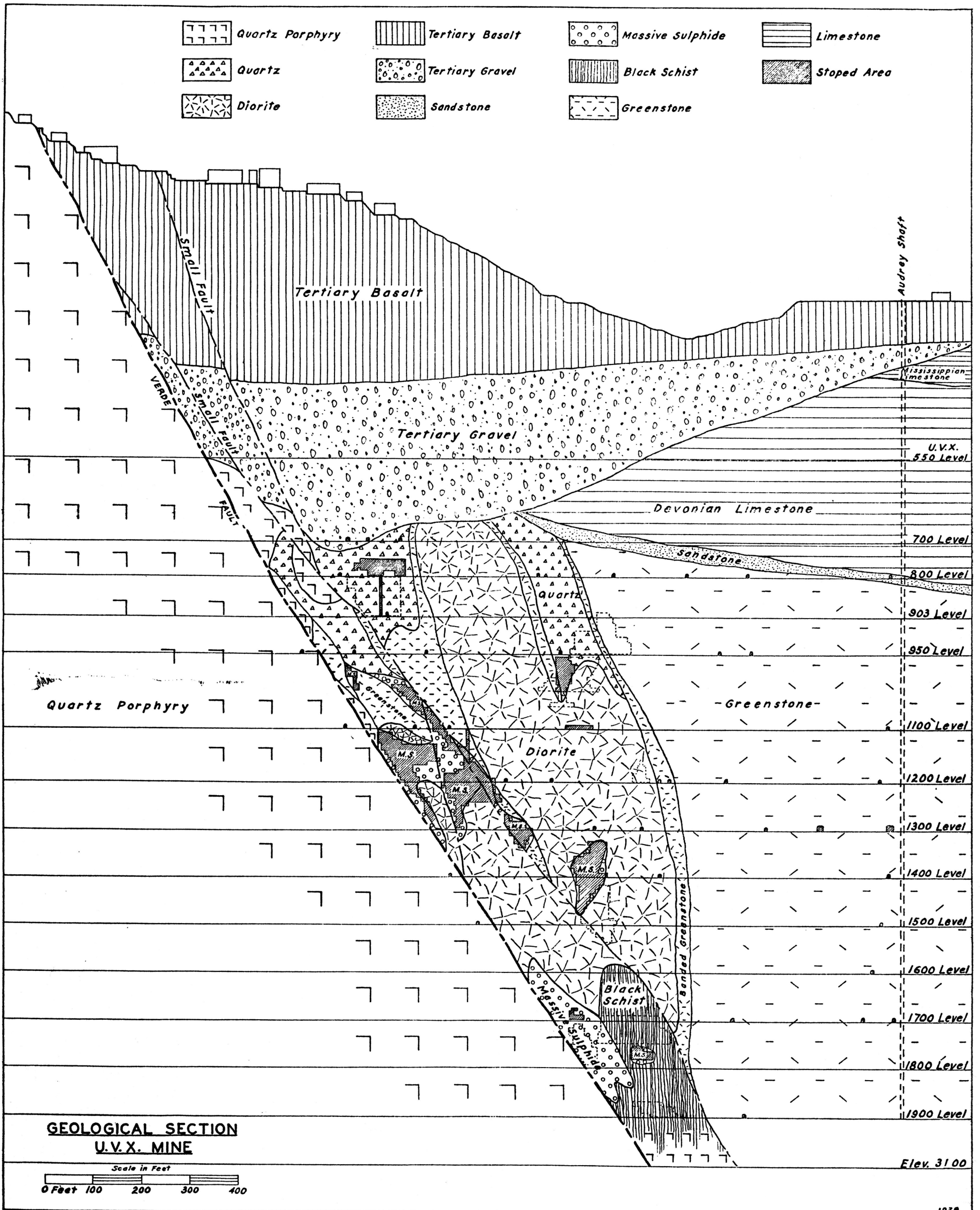
Plate XIV.—Geologic section through U.V.X. ore zone along line A-A' of Plate XIII. Section trends northeast and passes near Audrey shaft.
