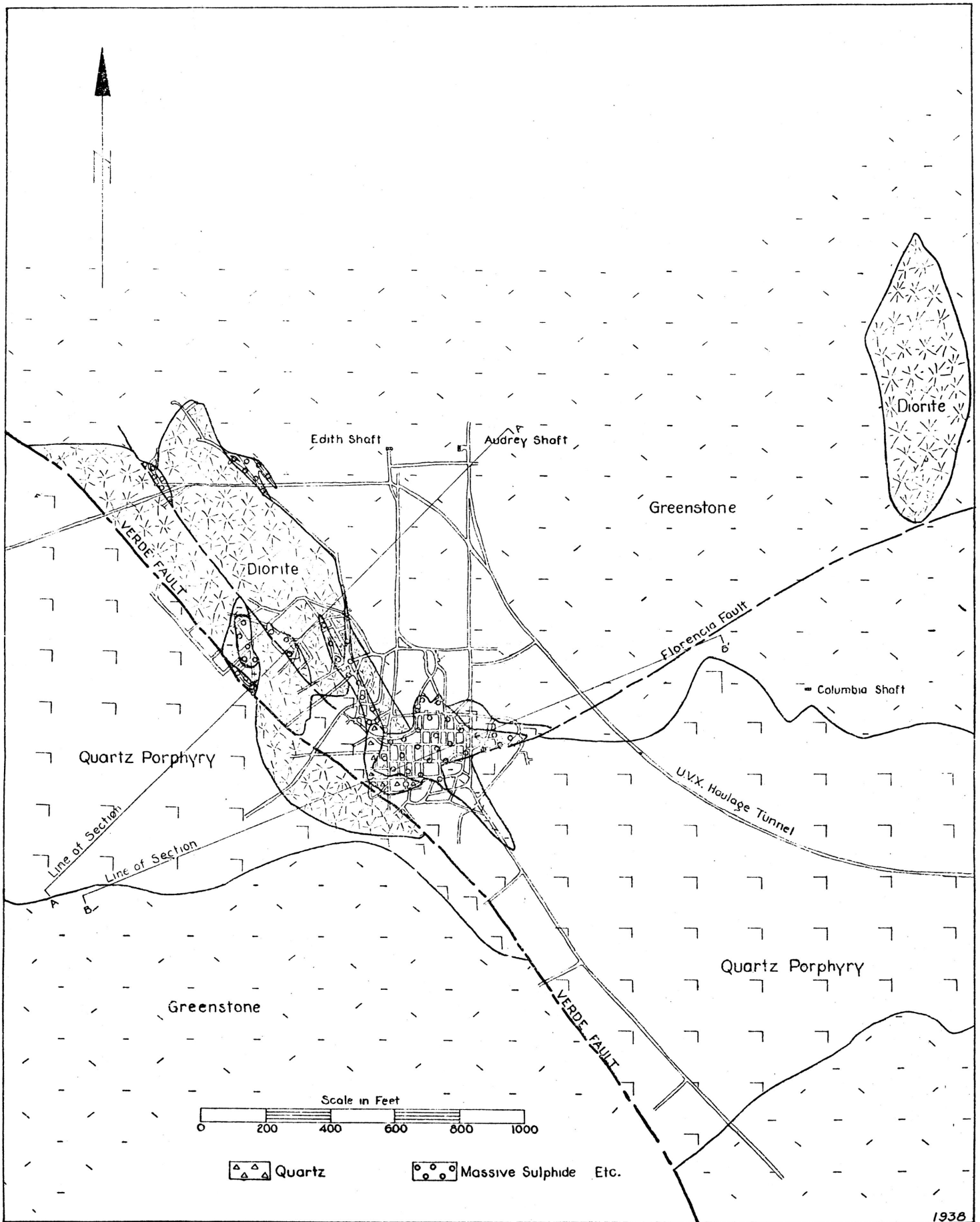
Plate XIII.—Generalized geologic map of United Verde Extension 1,300-foot level.
