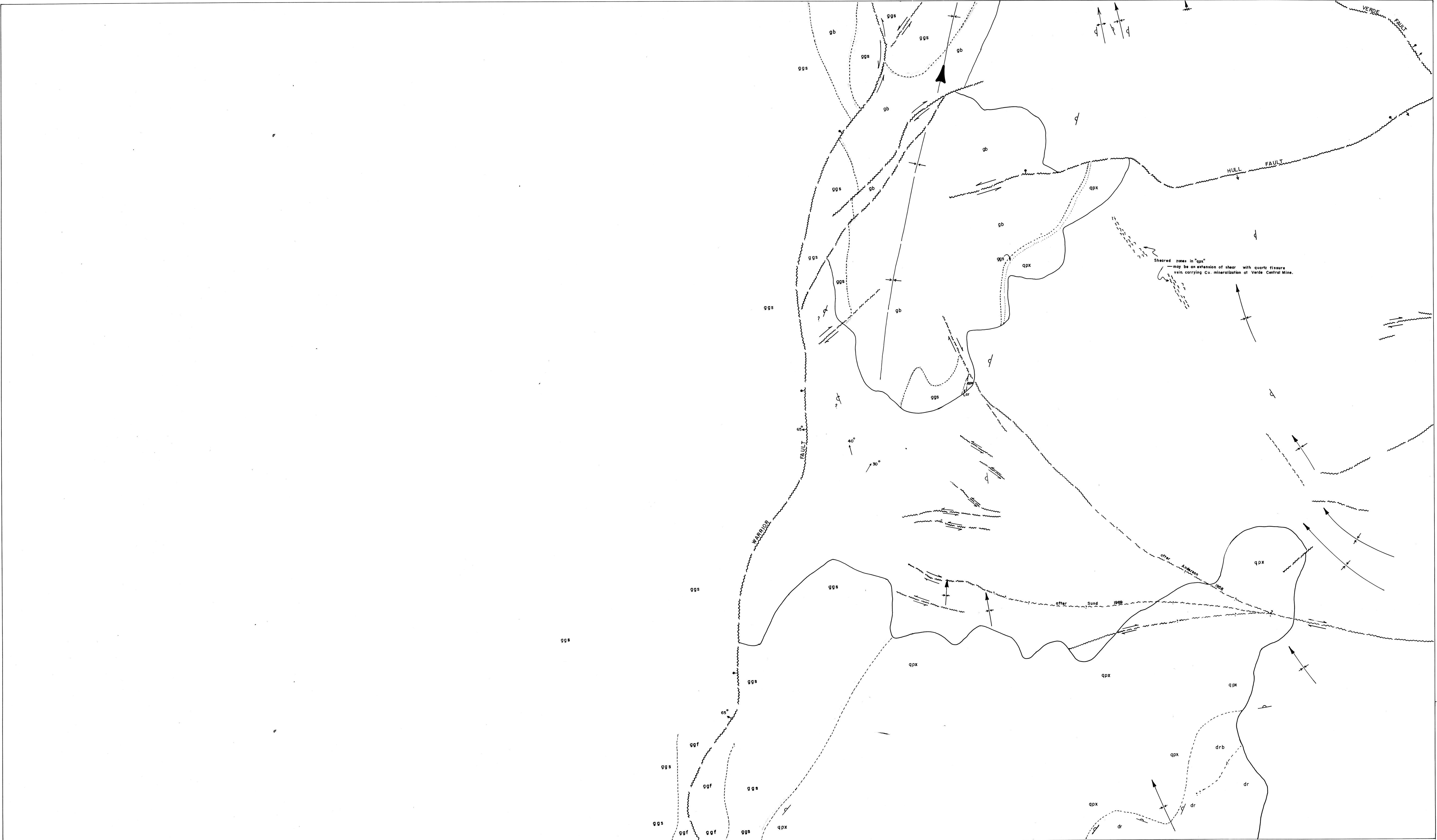
MM-4 OVERLAY SHOWING GEOLOGY INTERPRETED UNDER POST-PRECAMBRIAN COVER WITH STRUCTURAL INTERPRETATION
