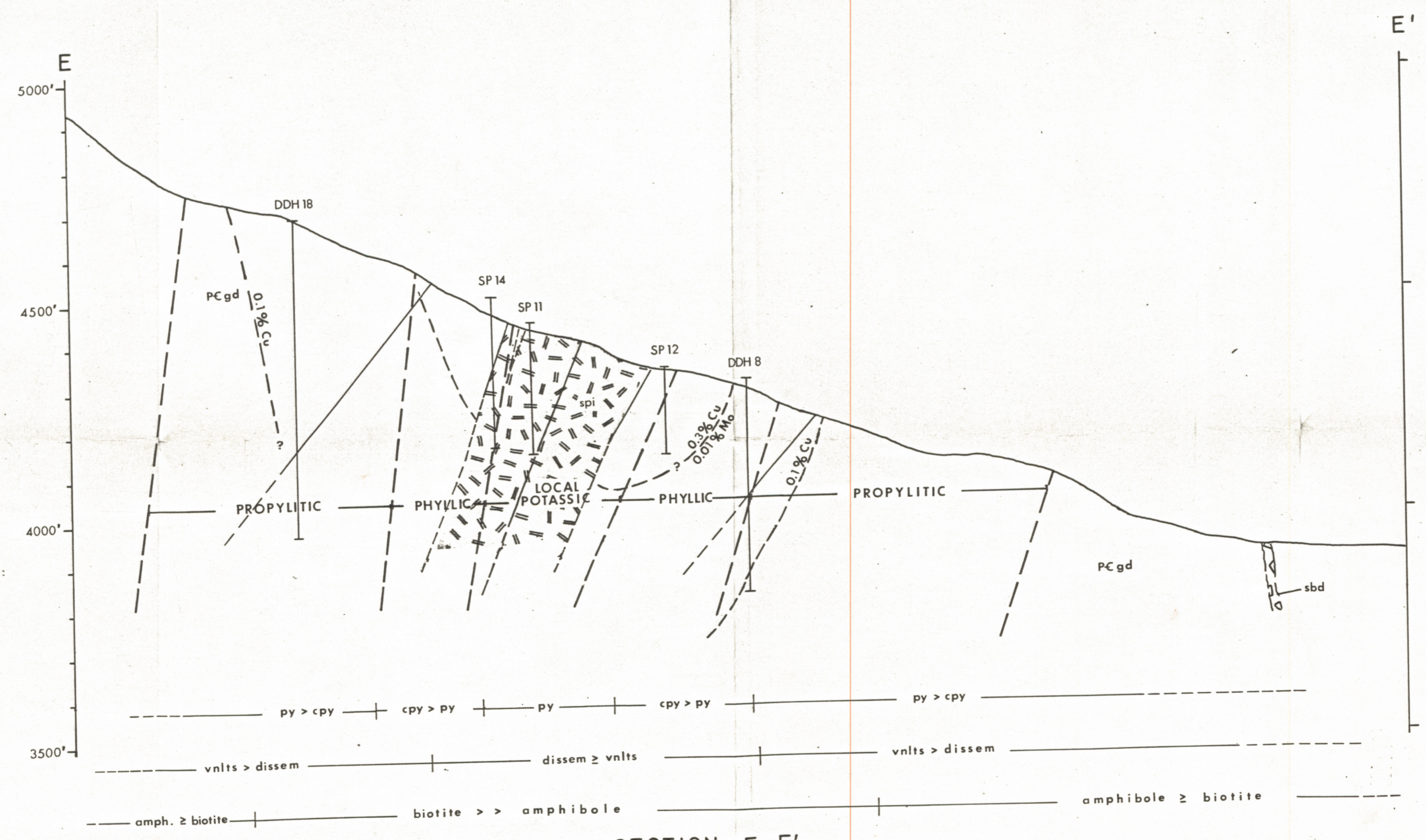
Figure 4 ALTERATION AND MINERALIZATION ZONING OF THE SQUAW PEAK PORPHYRY COPPER DEPOSIT
