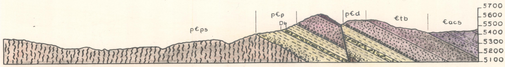
SECTION C-C'
