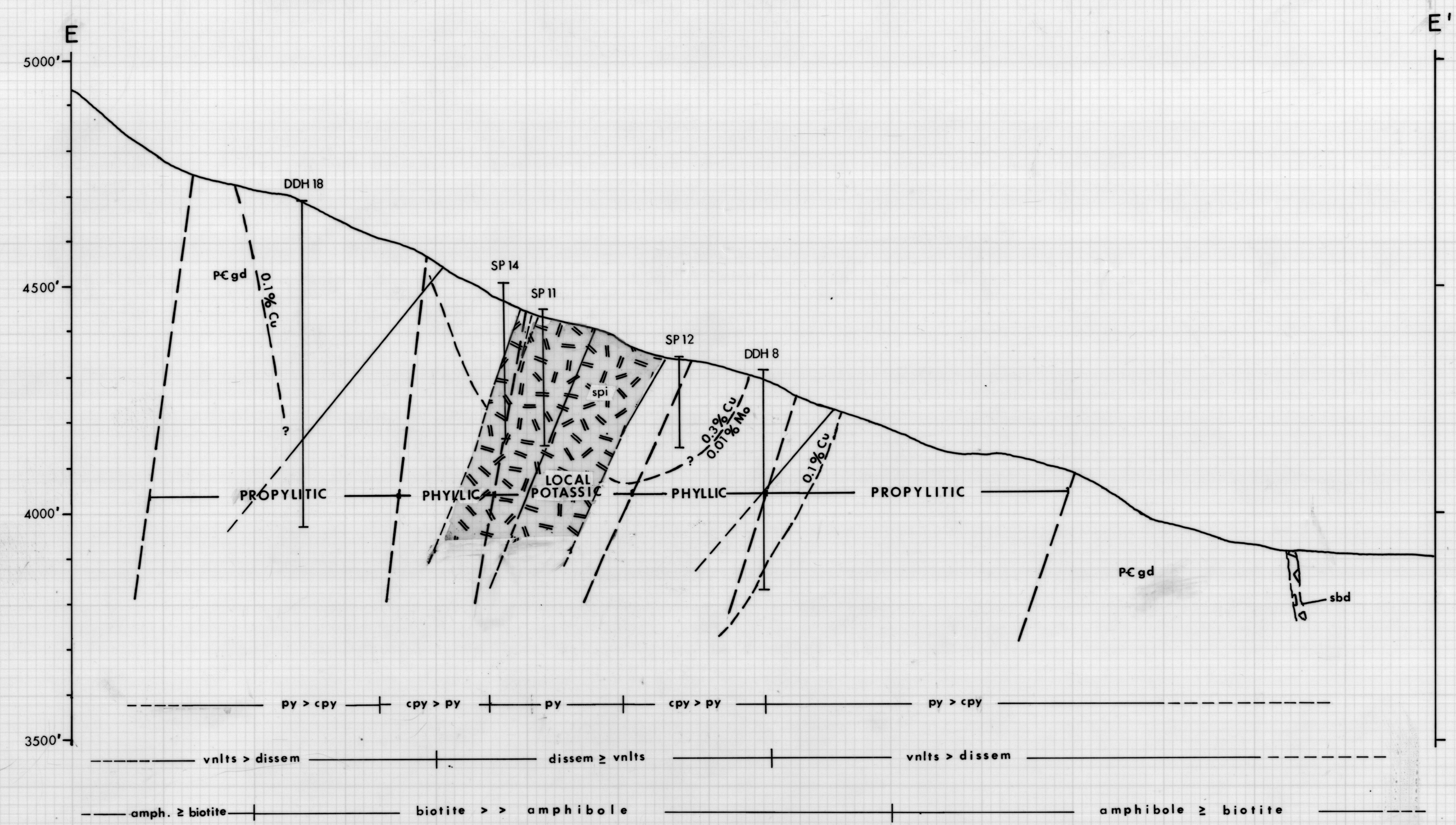
SECTION E-E' LOOKING NORTH
