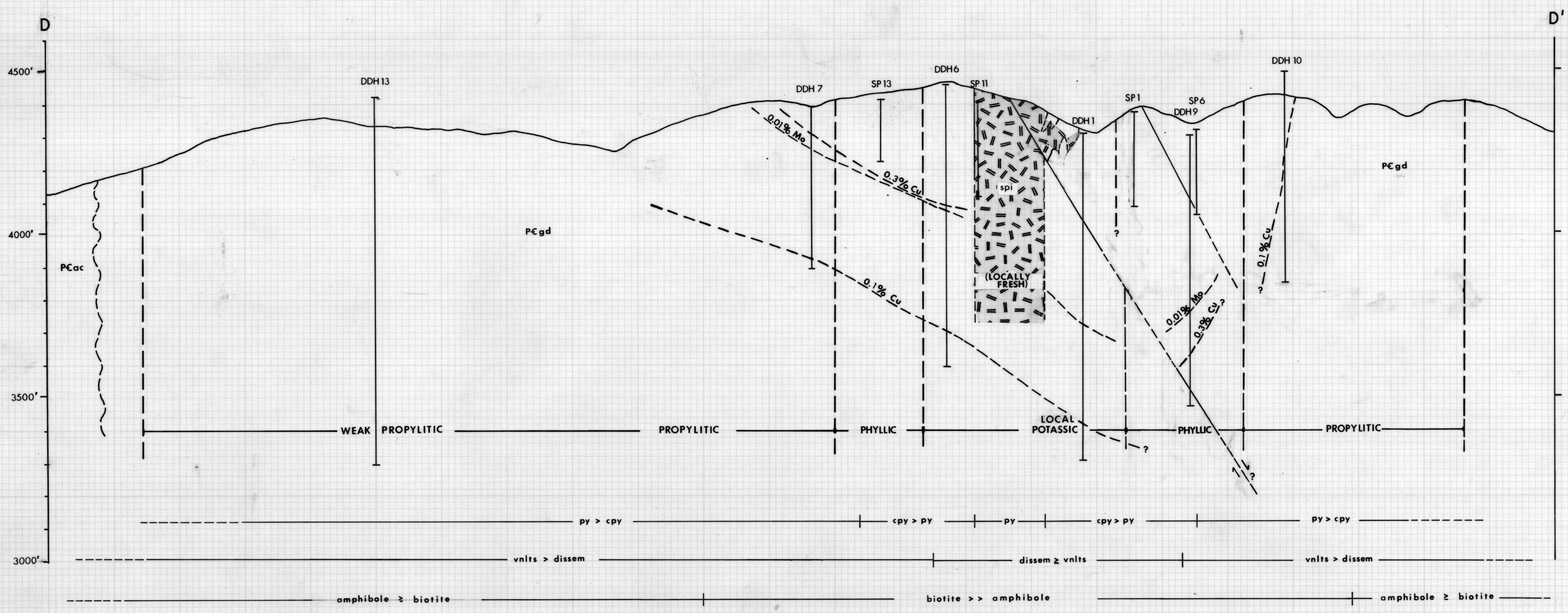
SECTION D-D' LOOKING EAST
