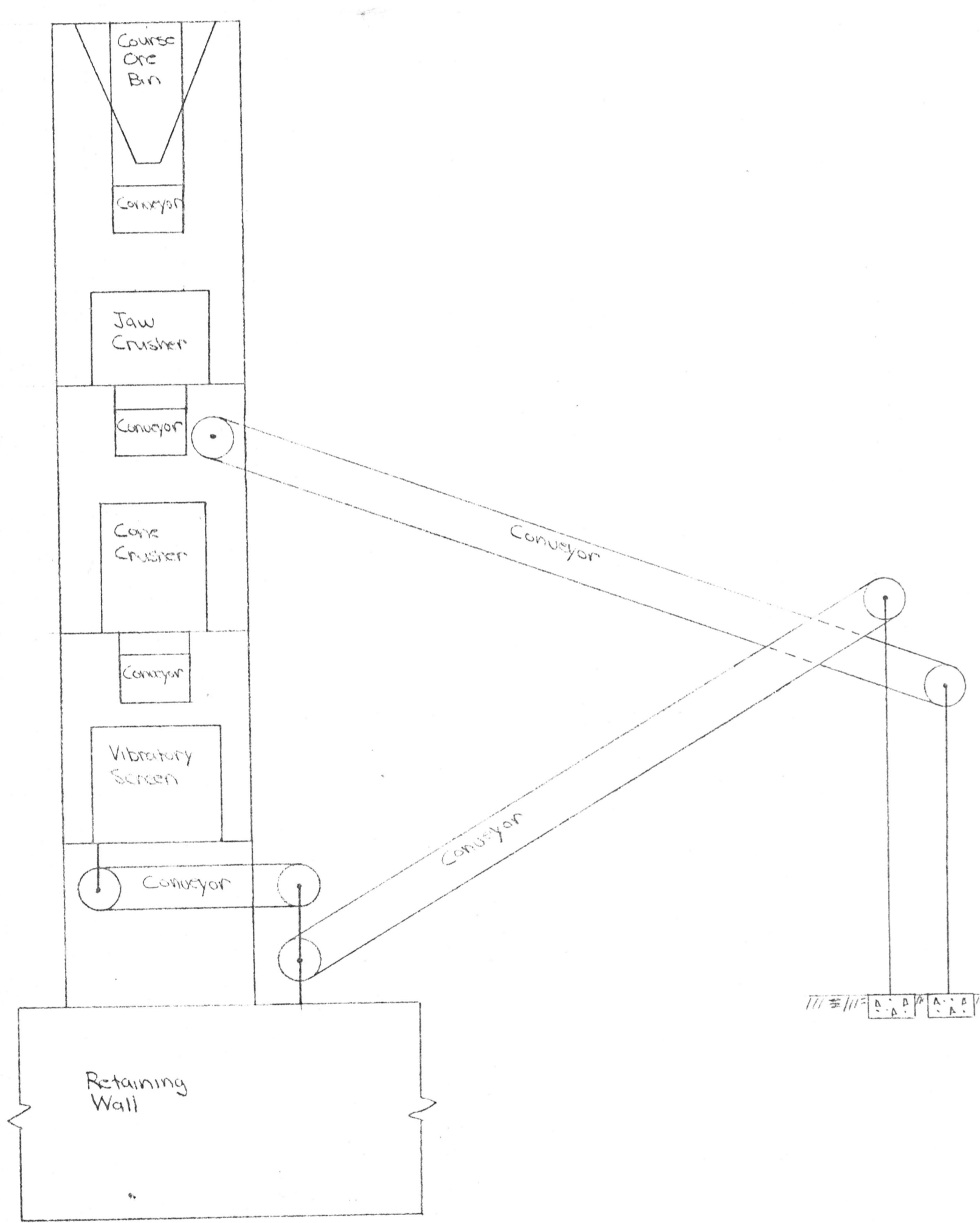
FRONT VIEW Scale: 1" = 5'
