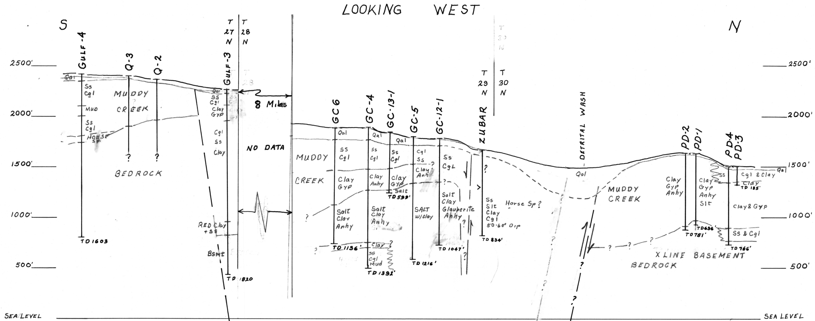
N-S CROSS SECTION THROUGH DRILL HOLES DETRITAL VALLEY, MOHAVE COUNTY, AZ
