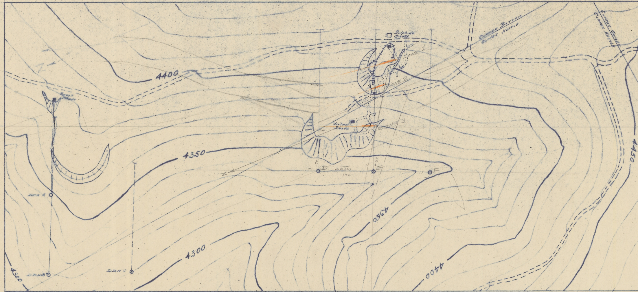
PLAN - SULPHIDE SHAFT AREA 100' LEVEL WORKINGS
