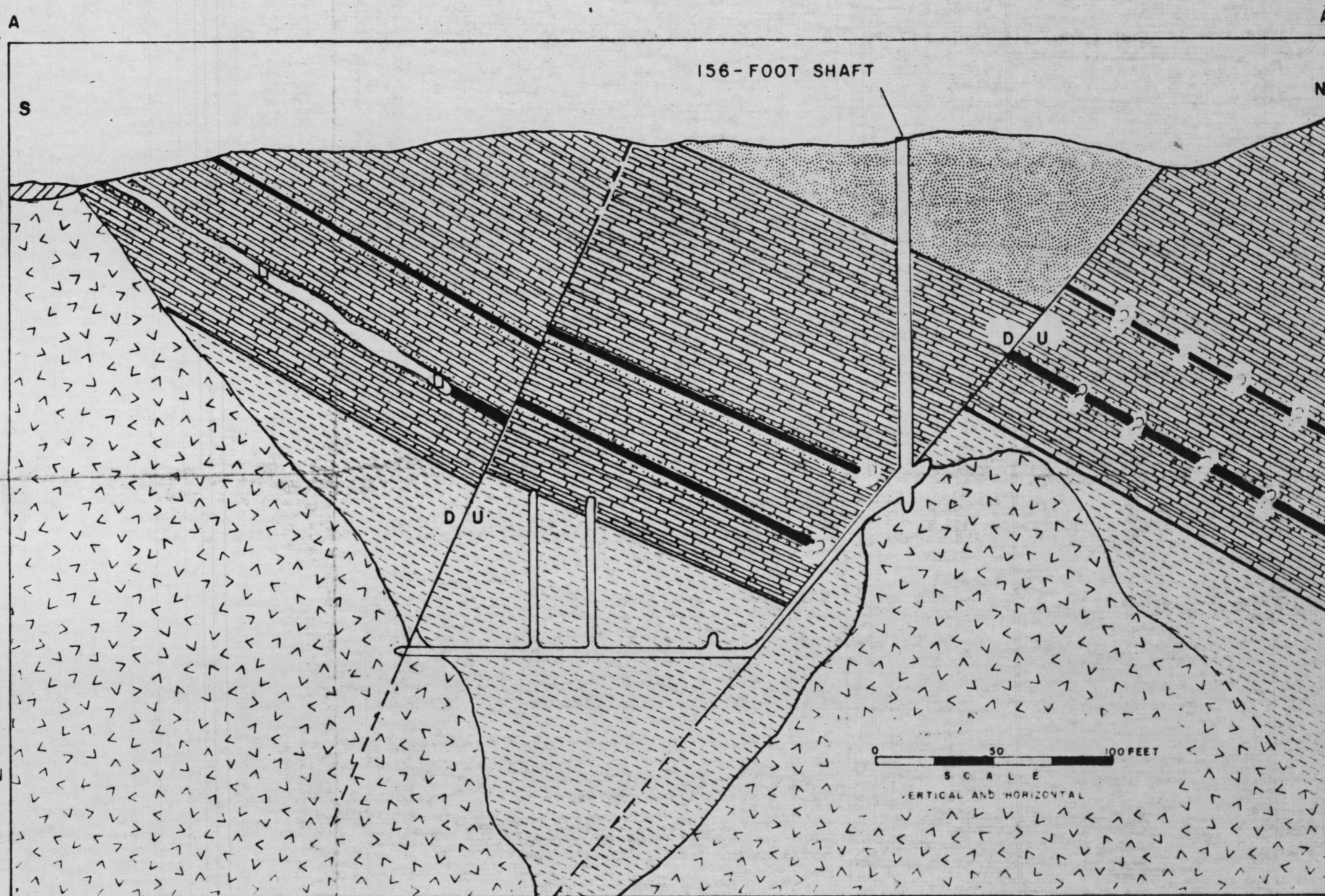
FIGURE 18 CROSS SECTION A-A' GOLDEN RULE MINE AREA, COCHISE COUNTY, ARIZONA, FACING WEST.-- MODIFIED FROM WUENSCH (1927)
