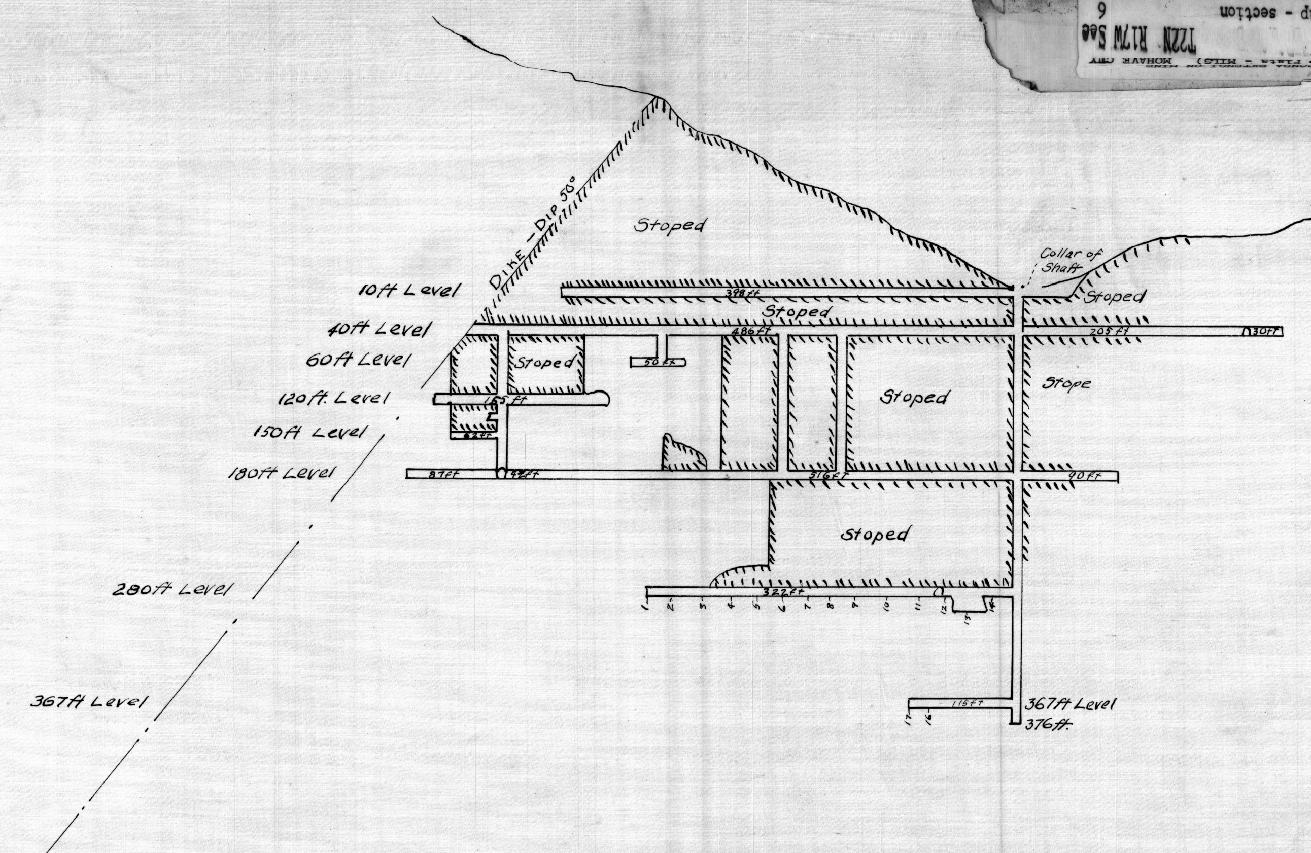
Section of the Underground Workings of the GOLCONDA EXTENSION MINE MOHAVE COUNTY, ARIZONA. Traced by: M.G. Gullety
