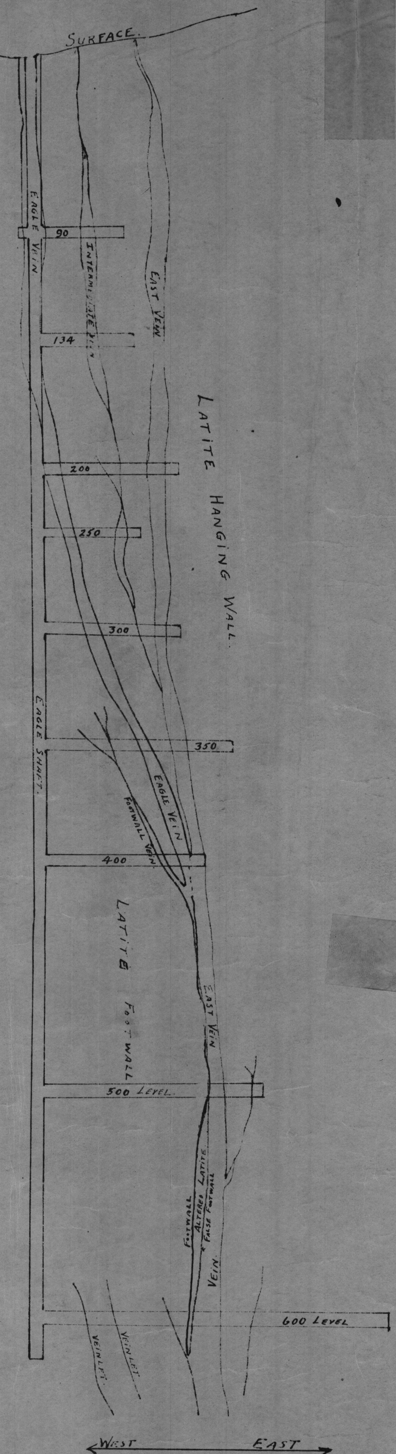
CROSS SECTION OF THE EAGLE MINE THRU EAGLE SHAFT SCALE 1"=40 FT
