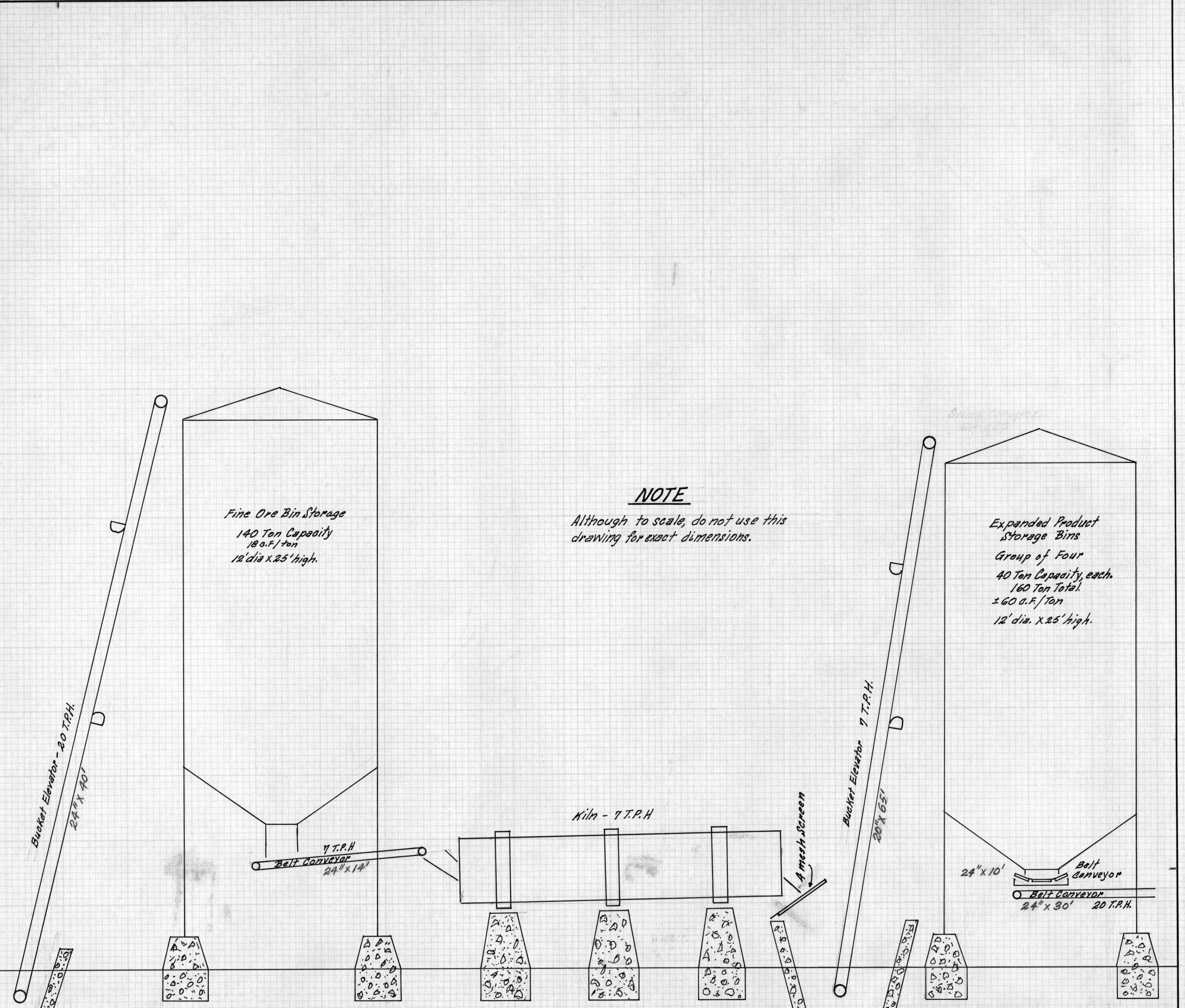
Process Plant Elevation Scale: 1/4" = 1 Ft. 1" = 4 Ft.
