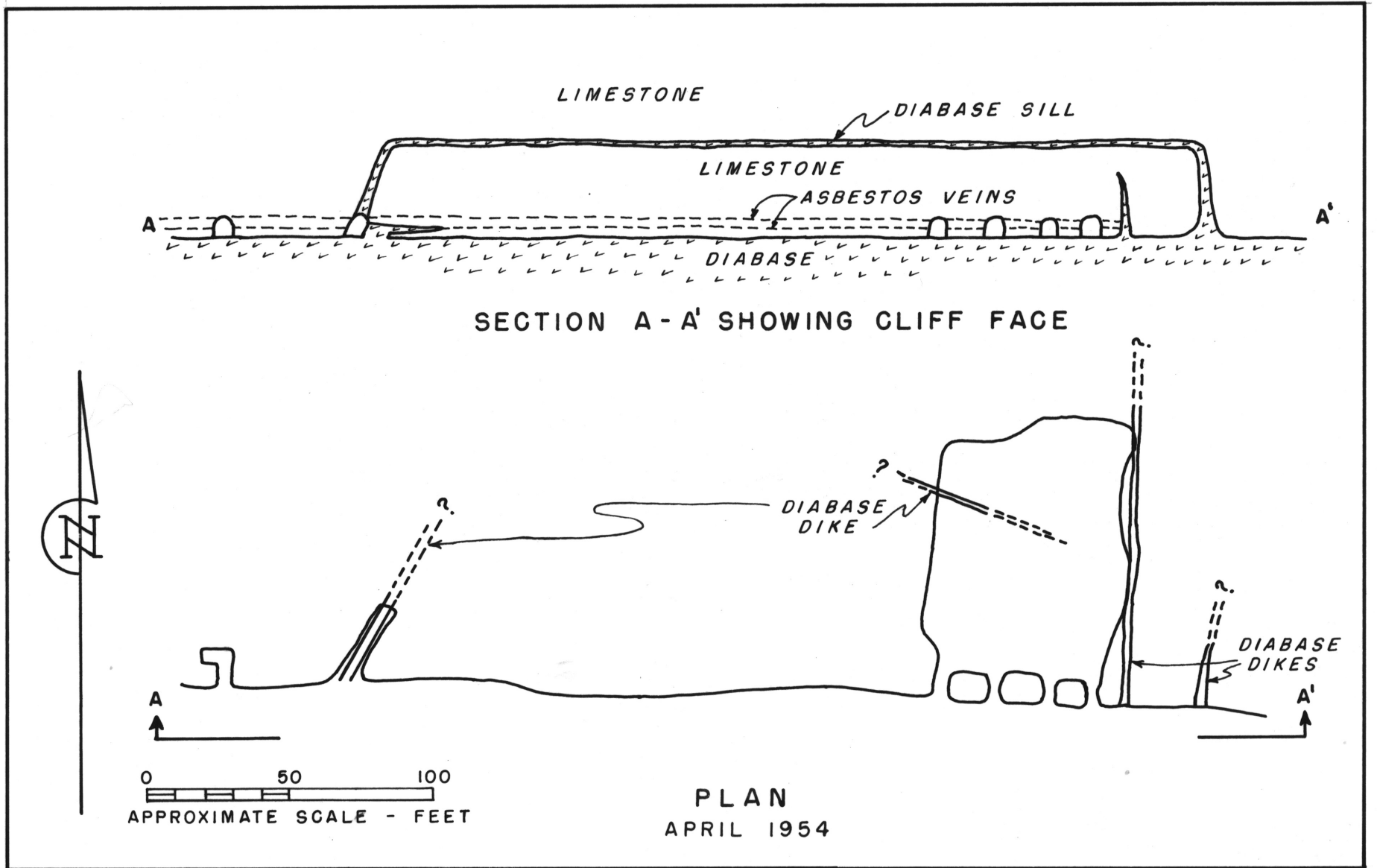
FIGURE 33. - SKETCH MAP - MAN O' WAR MINE - MELROSE MINES
