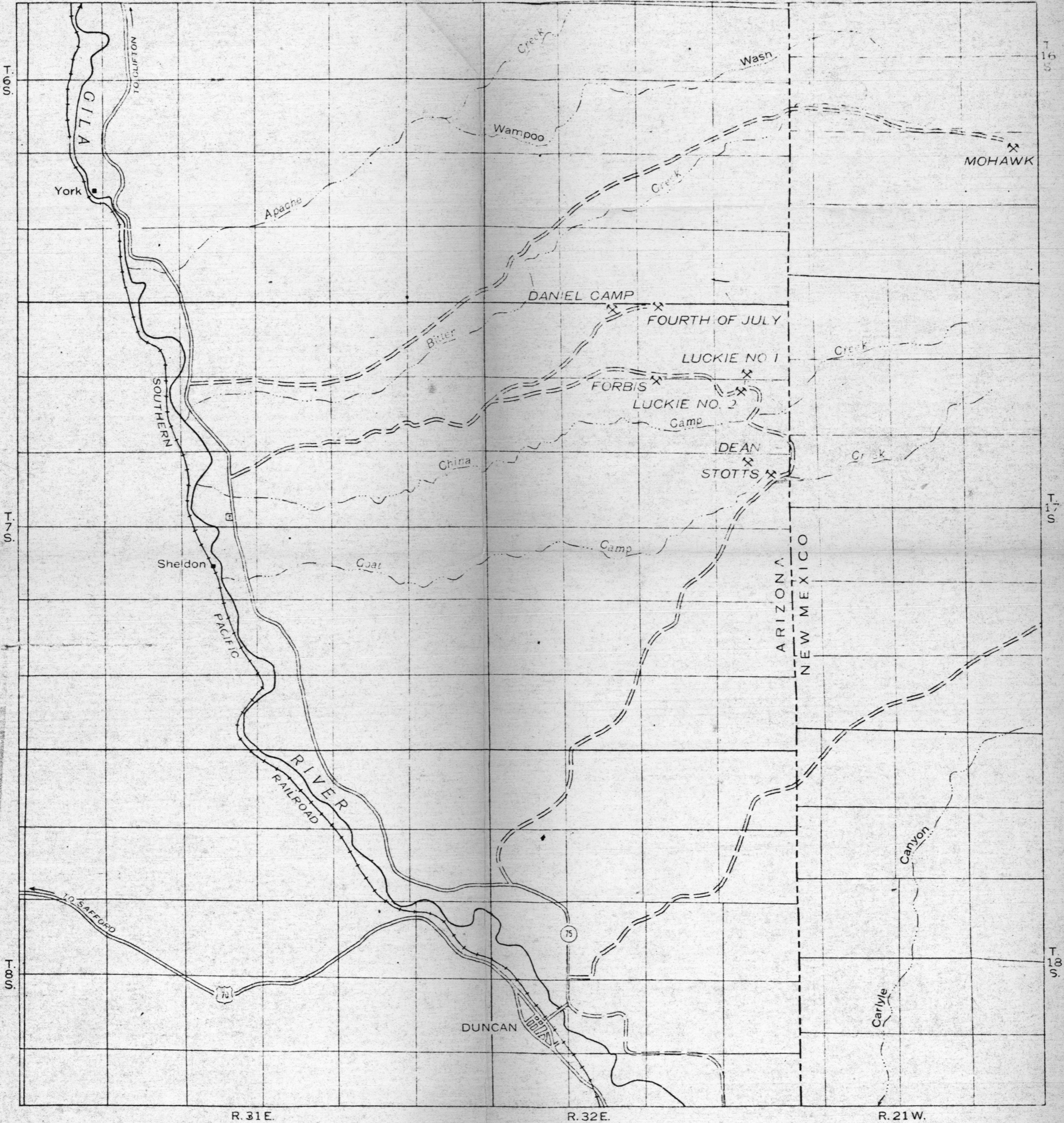
INDEX MAP SHOWING LOCATION OF FLUORSPAR DEPOSITS NEAR DUNCAN, GREENLEE COUNTY, ARIZONA
