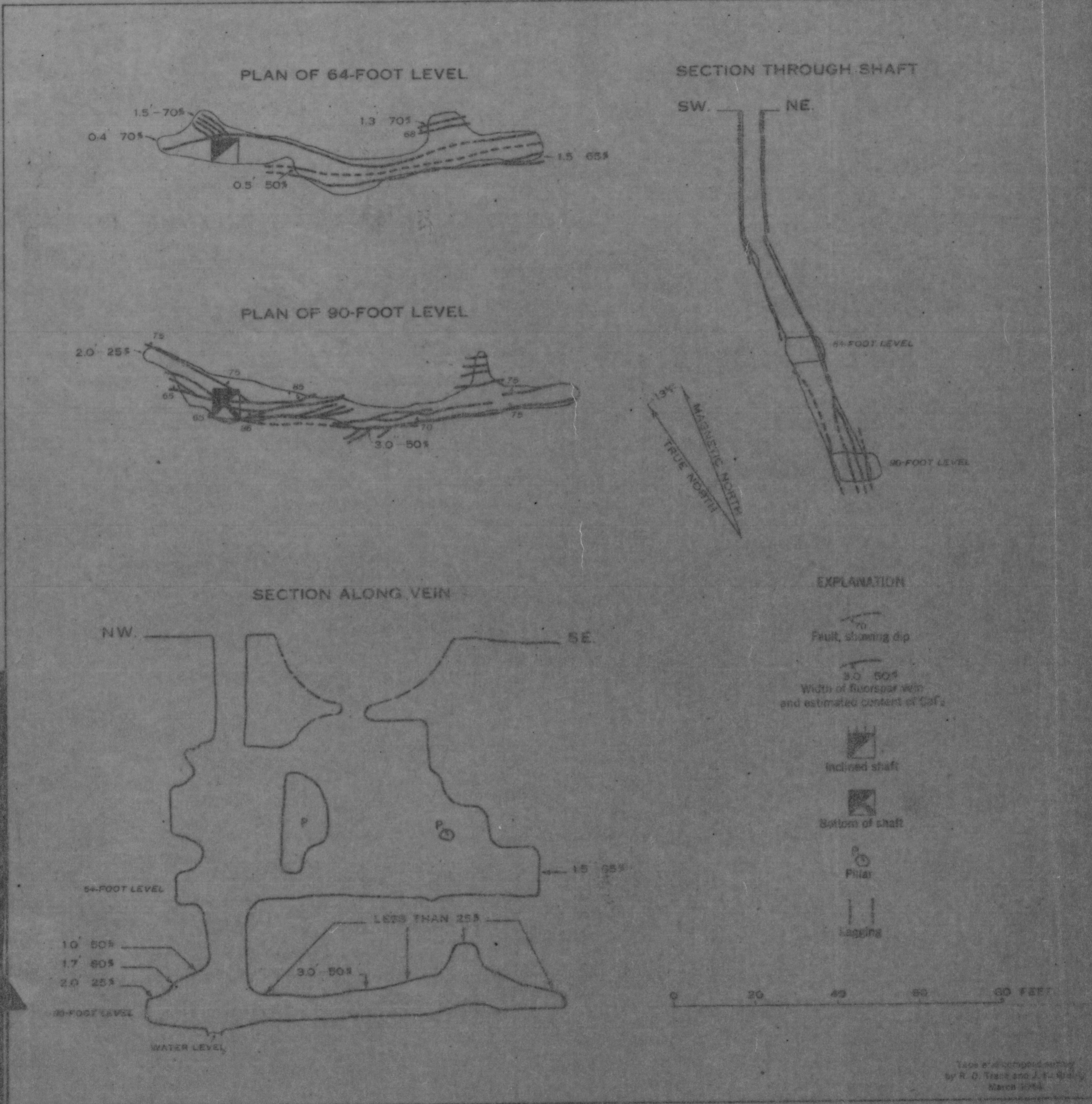
LEVEL MAPS AND SECTIONS, LUCKIE NO. 2 FLUORSPAR MINE, GREENLEE COUNTY, ARIZONA
