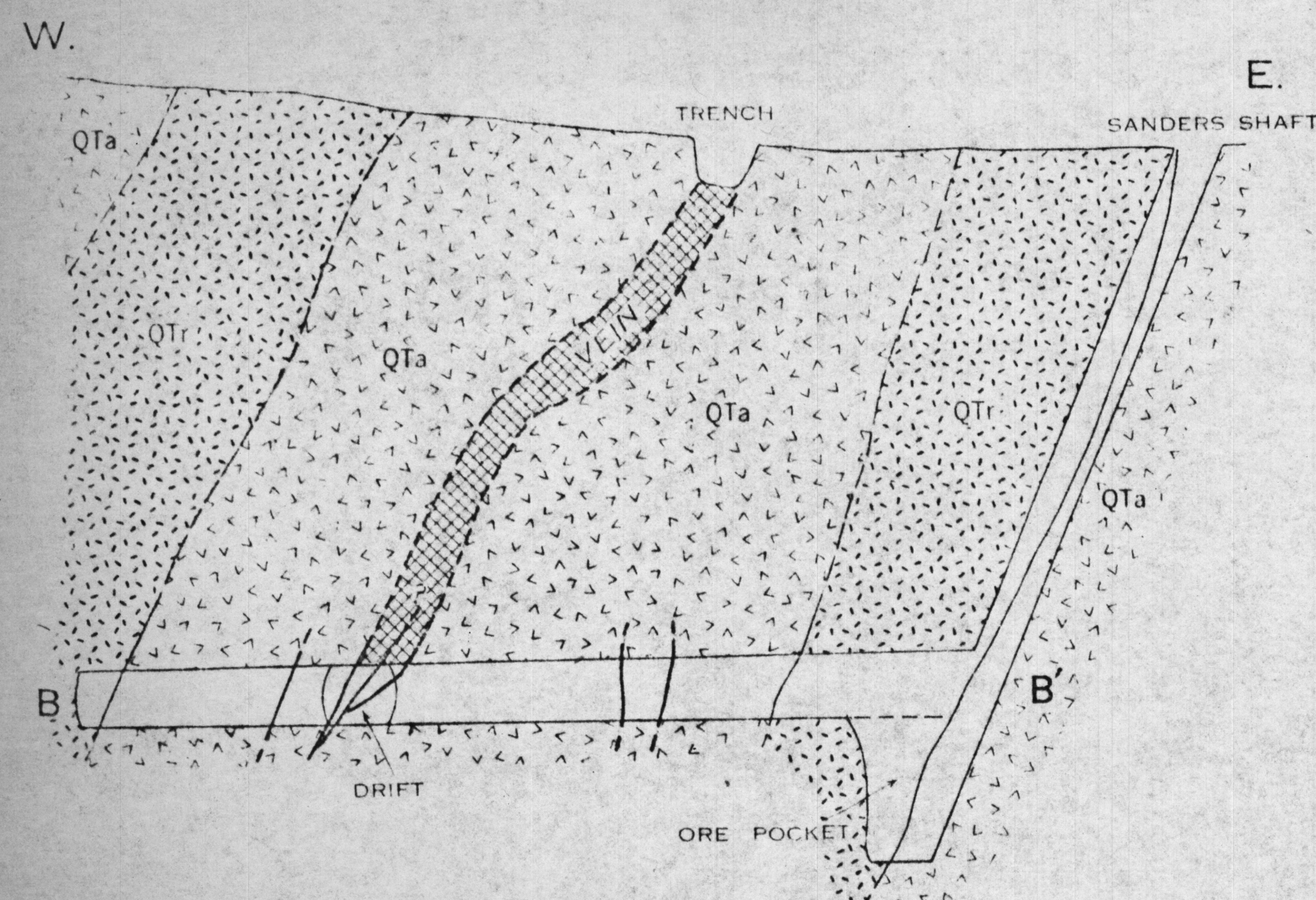
CROSS SECTION THROUGH SANDERS SHAFT
