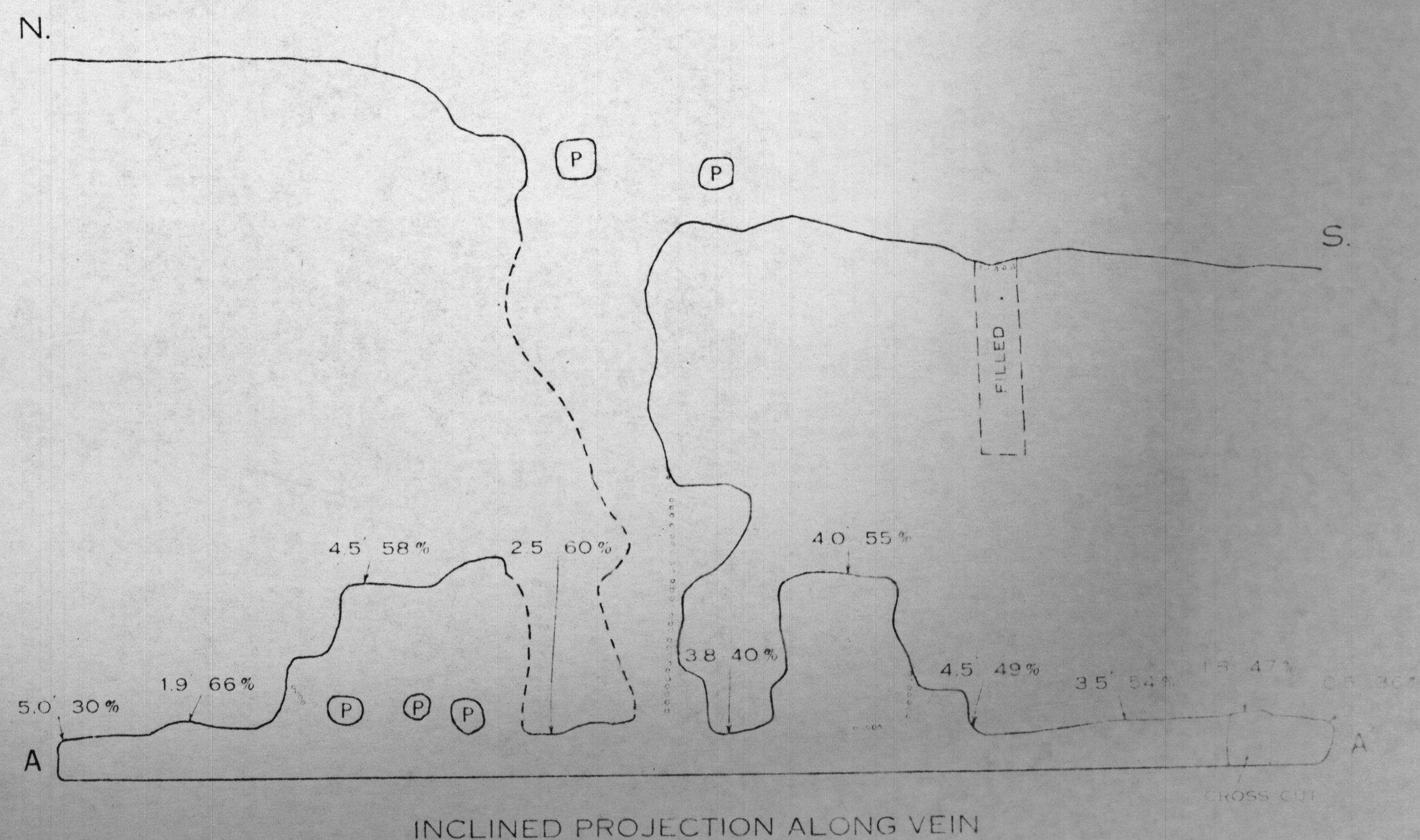
INCLINED PROJECTION ALONG VEIN
