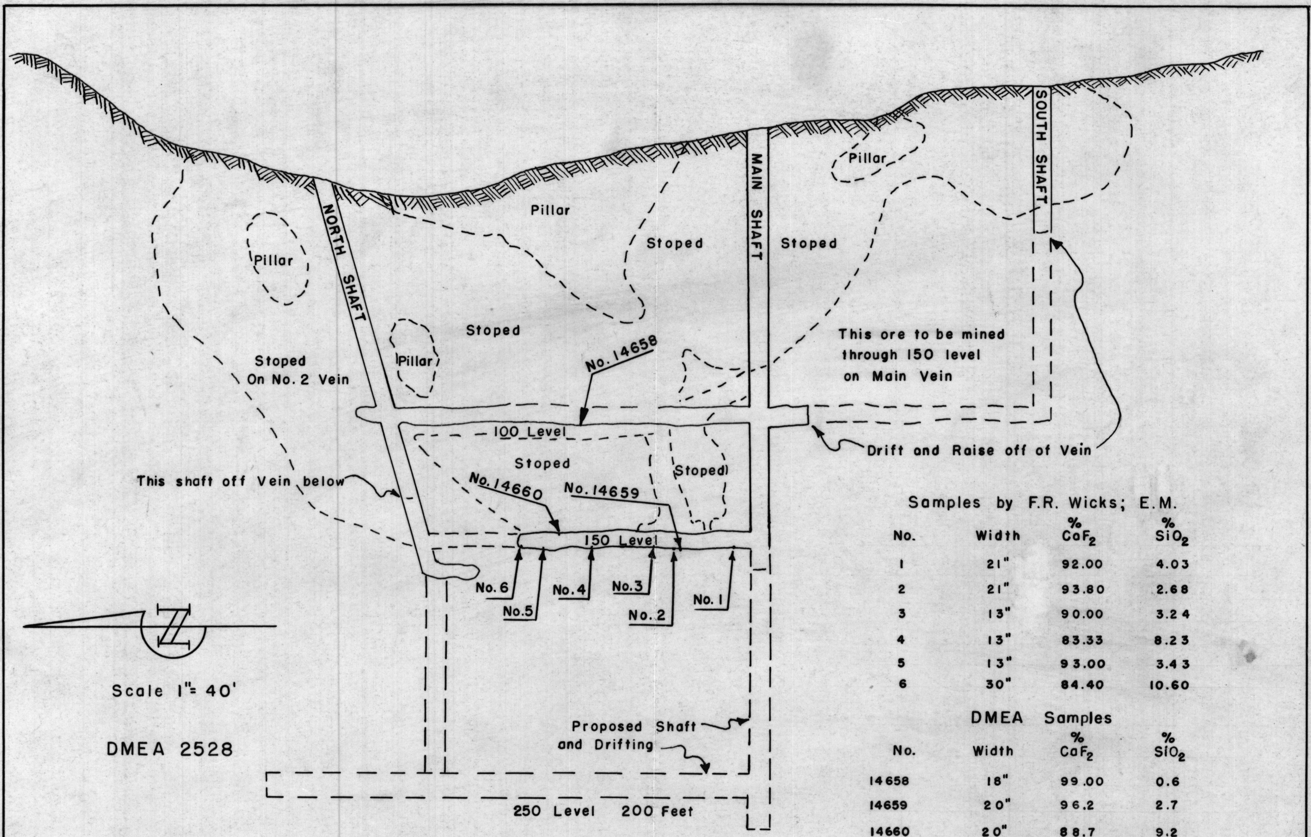
Figure 3 — Longitudinal Projection, Polly Anne Fluorspar Mine Greenlee County, Arizona
