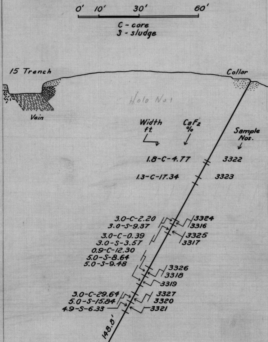
FIG. 4 - SECTION THROUGH DRILL HOLE SHOWING CaF 2 ASSAYS
