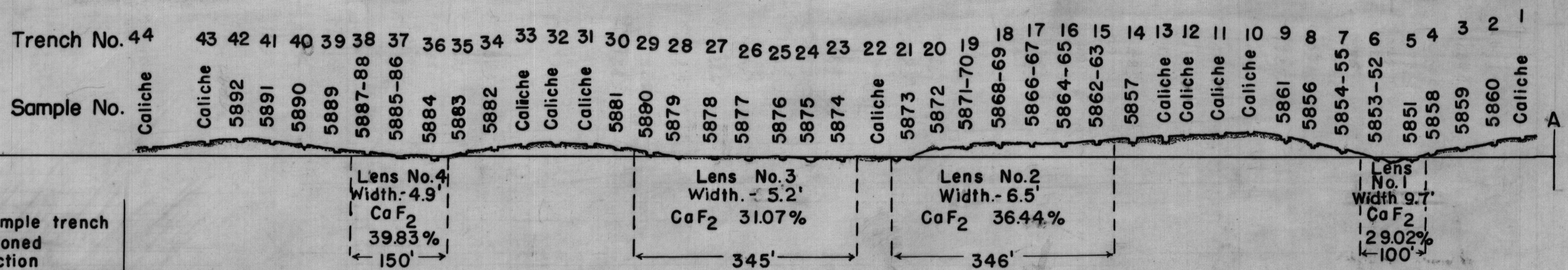
LONGITUDINAL SECTION ALONG STRIKE NEAR A-BD LENSES LOCATIONS
