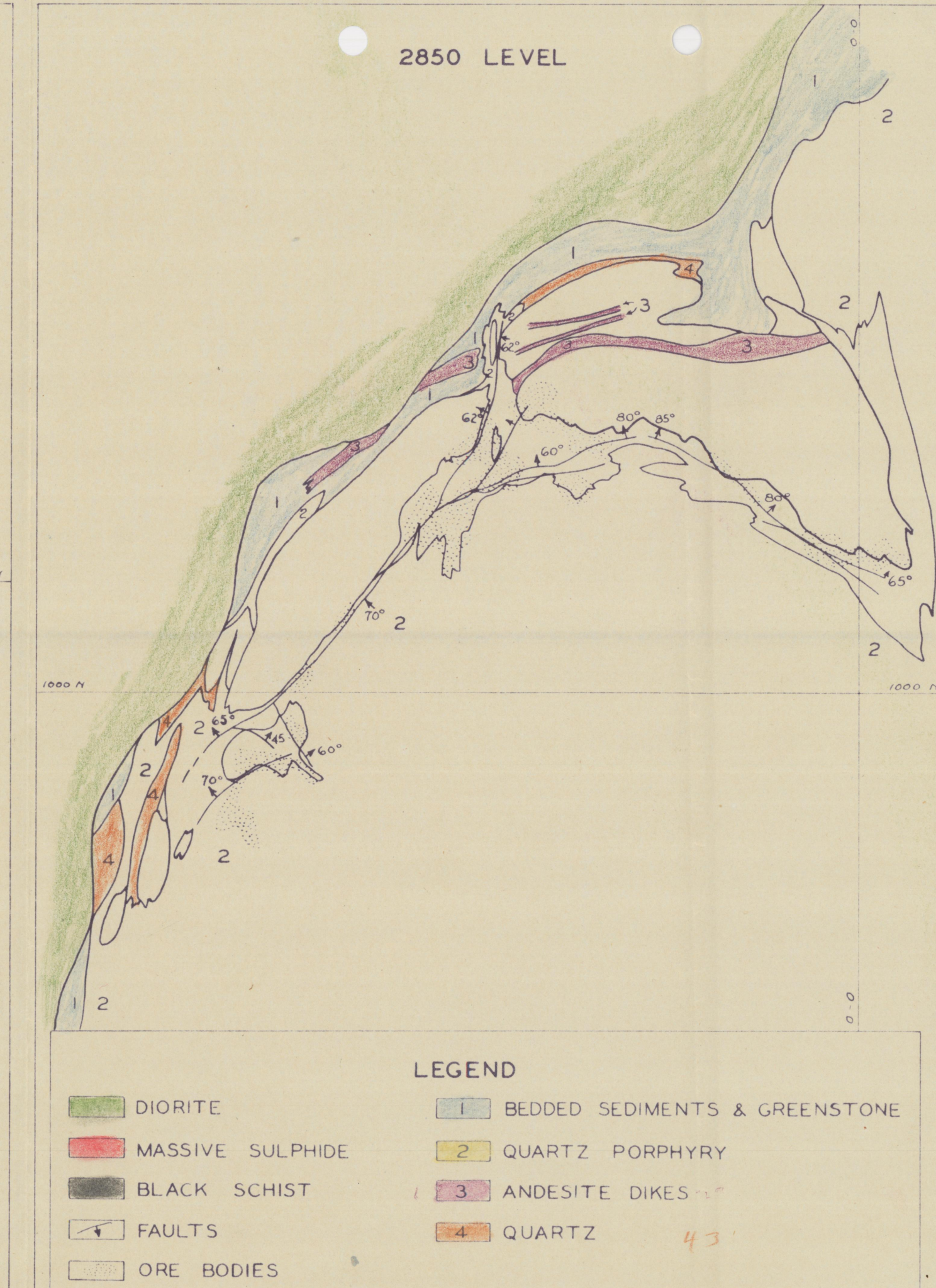
UNITED VERDE MINE CHANGES IN FORM AND SIZE OF SULPHIDE ZONE AND DISTRIBUTION OF ORE WITH INCREASING DEPTH 1" = 200'
