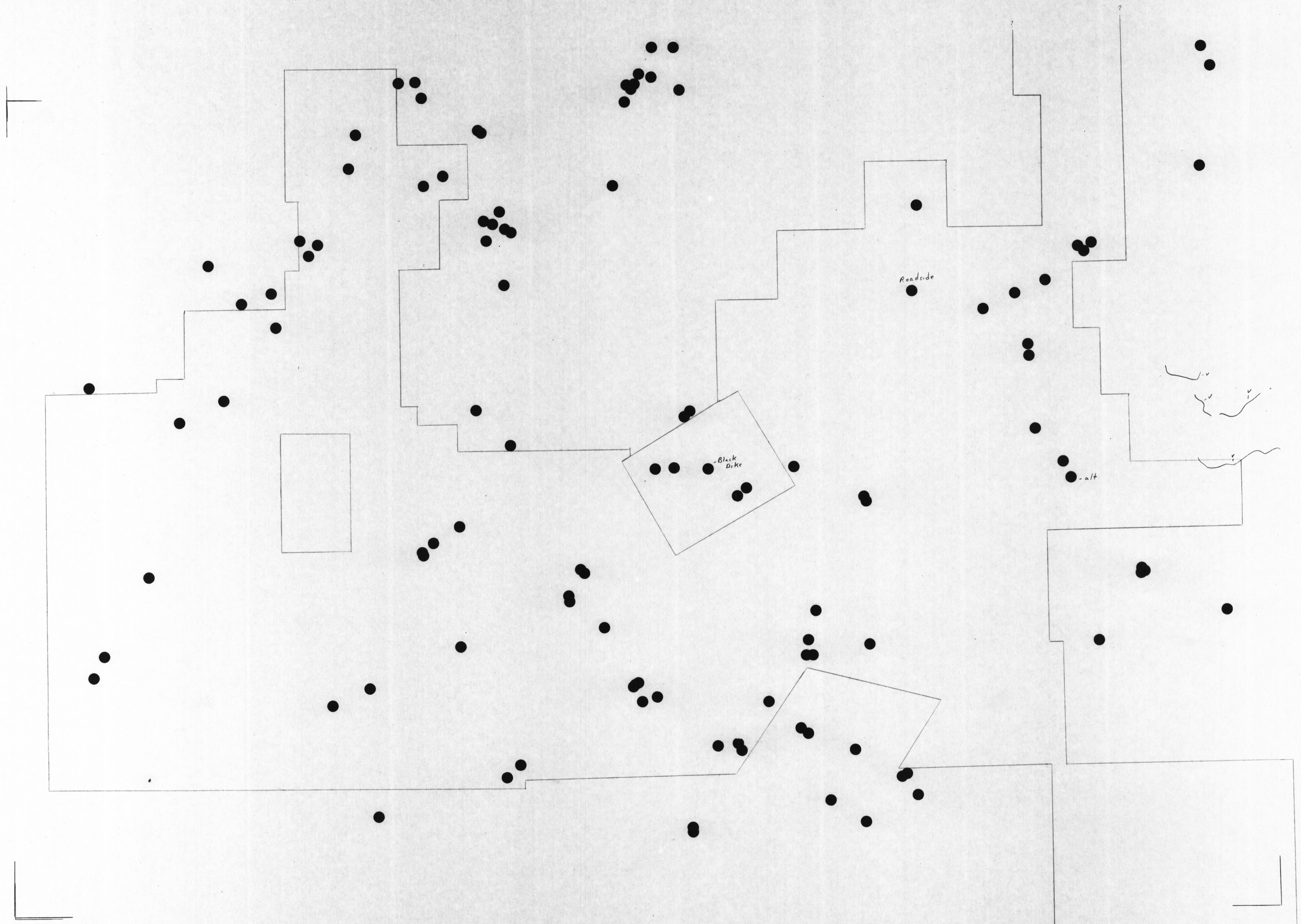
Land Status Map Roadside Project Map of Prospects and Mineralized Outcrops - Roadside Mine Area For Ivy Minerals For Ivy Minerals by P. O'Hara December, 1987
