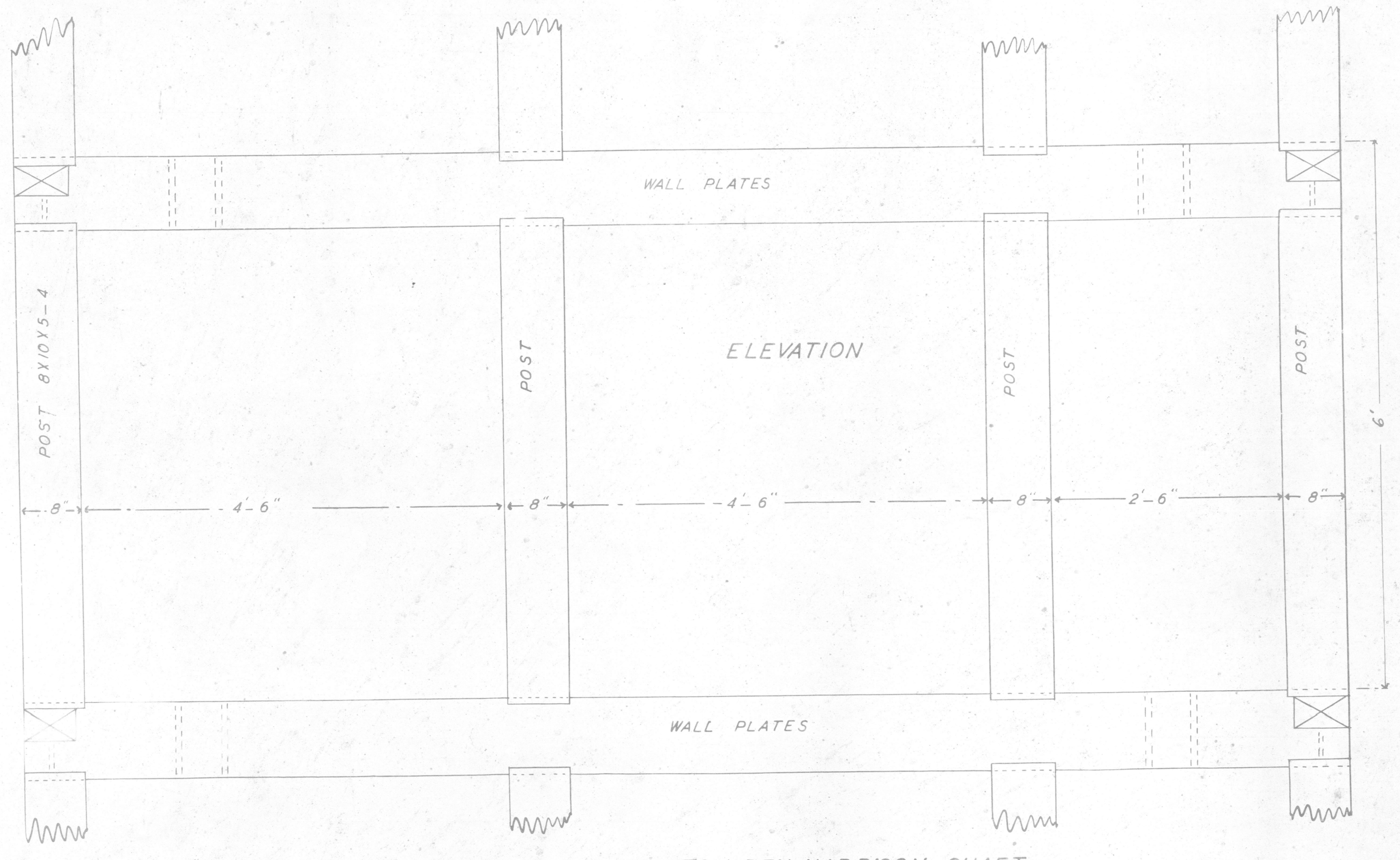
DETAILS OF SHAFT SETS - BEN HARRISON SHAFT TOM REED GOLD MINES COMPANY OATMAN - ARIZONA
