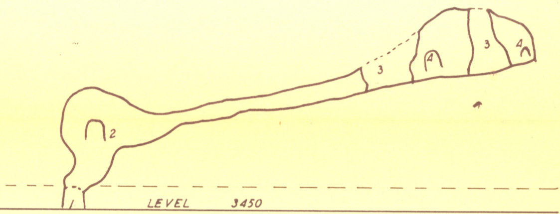
A-A SECTION THROUGH VANADIUM STOPE 1- X-CUT EL. 3450 2- X-CUT EL. 3464 3- PILLAR 4- CONNECTION TO LEAD STOPE
