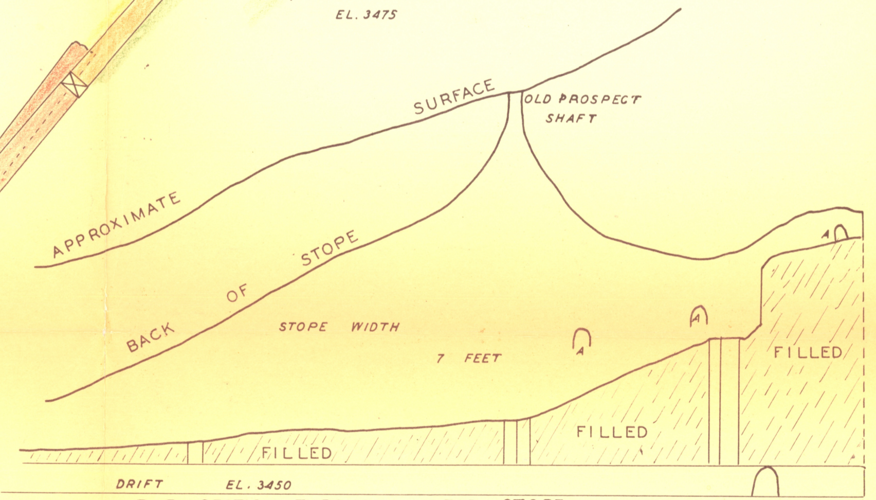
B-B SECTION THROUGH LEAD STOPE A - CONNECTION TO VANADIUM STOPE
