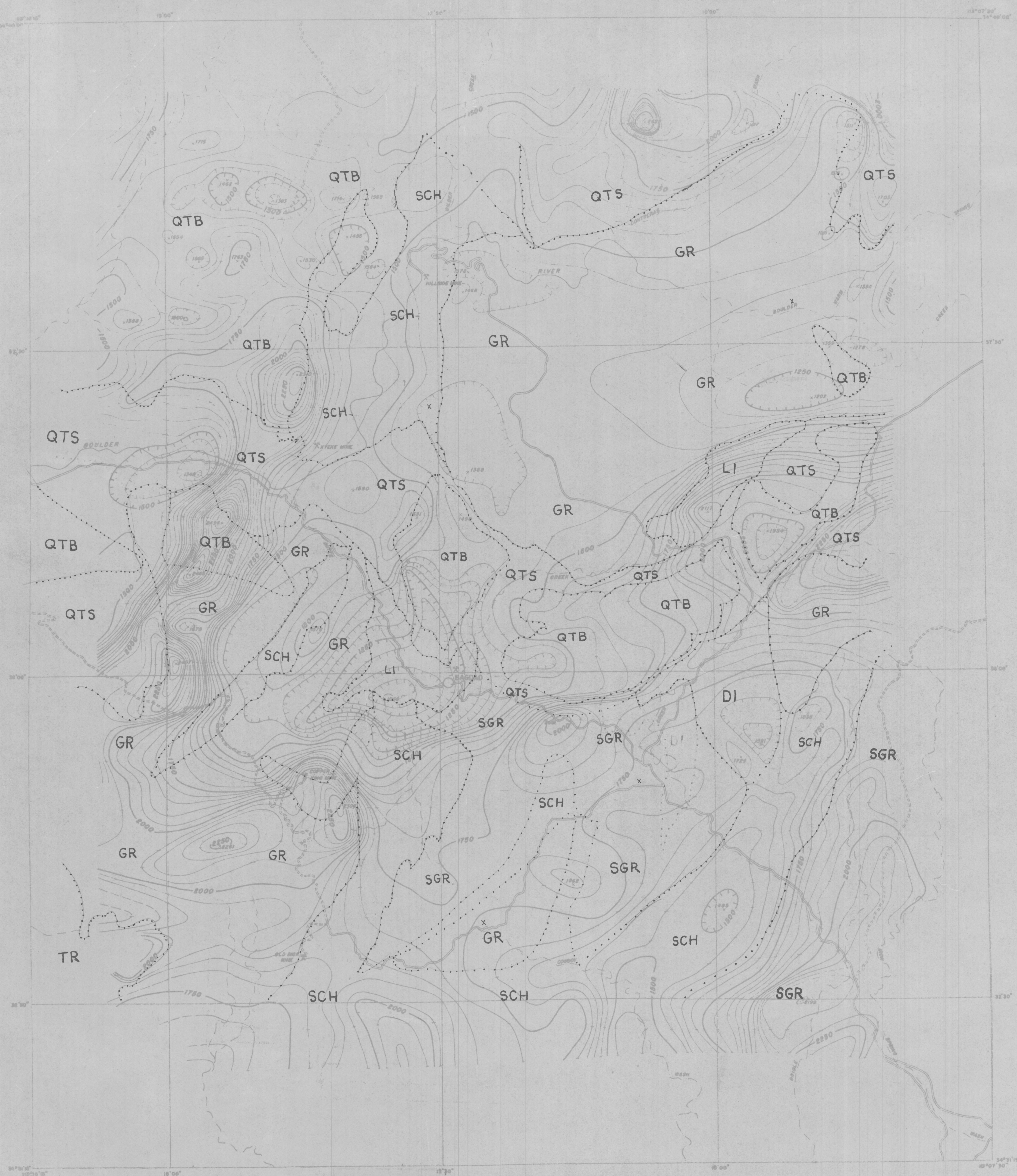
TOTAL INTENSITY AEROMAGNETIC MAP OF THE BAGDAD AREA, YAVAPAI COUNTY, ARIZONA
