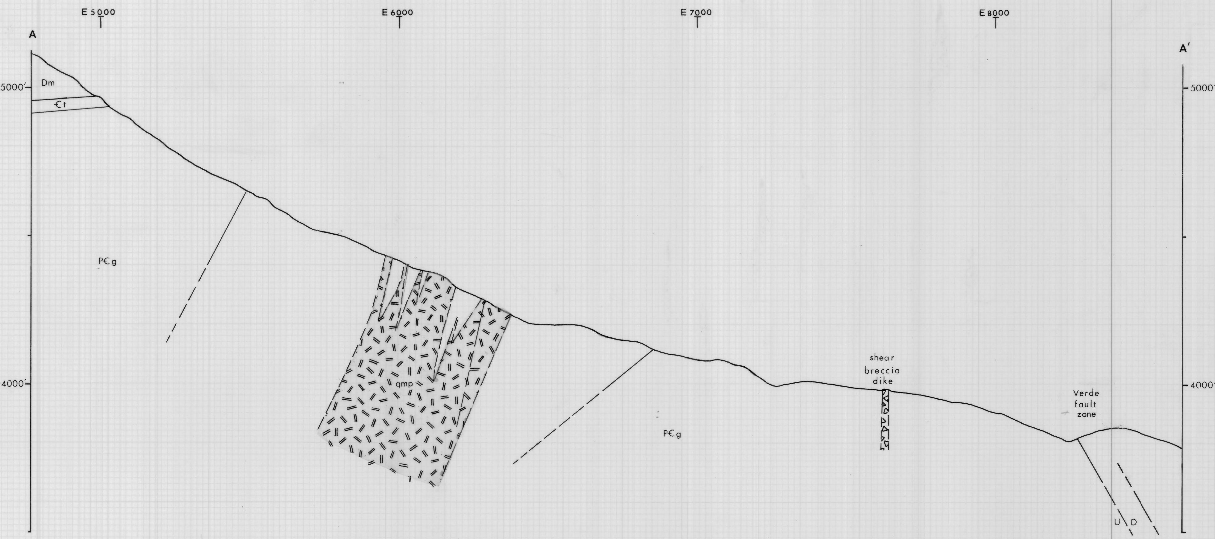
GEOLOGIC SECTION A - A' LOOKING NORTH ONE INCH EQUALS 200 FEET
