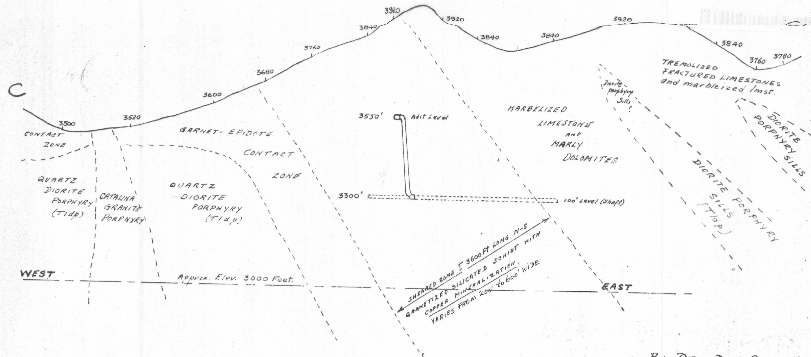
CATALINA, SUNNYSIDE AND ORBIT CLAIMS E - W SECTION THROUGH "C" - "D" WITH INFERRED GEOLOGY SCALE 1" = 200 FT.
