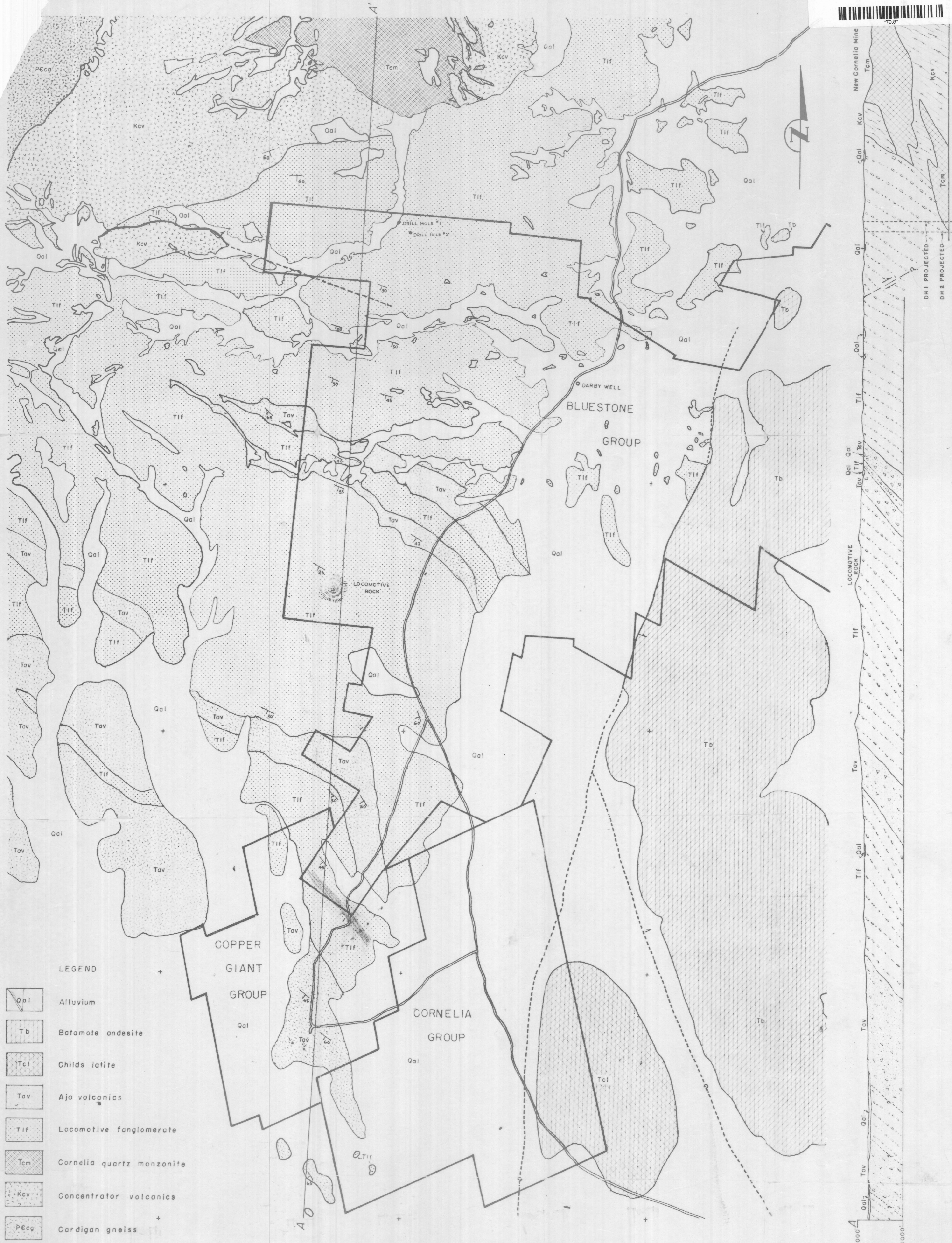
GEOLOGIC MAP & SECTION OF PART OF THE AJO MINING DISTRICT, PIMA COUNTY, ARIZONA (Modified after USGS)
