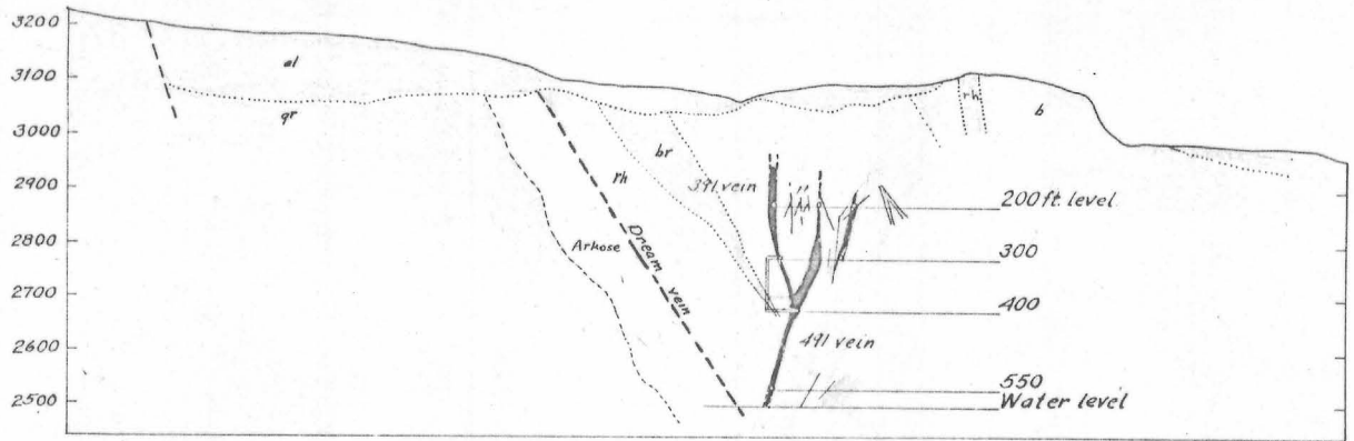
SECTION E-E'
