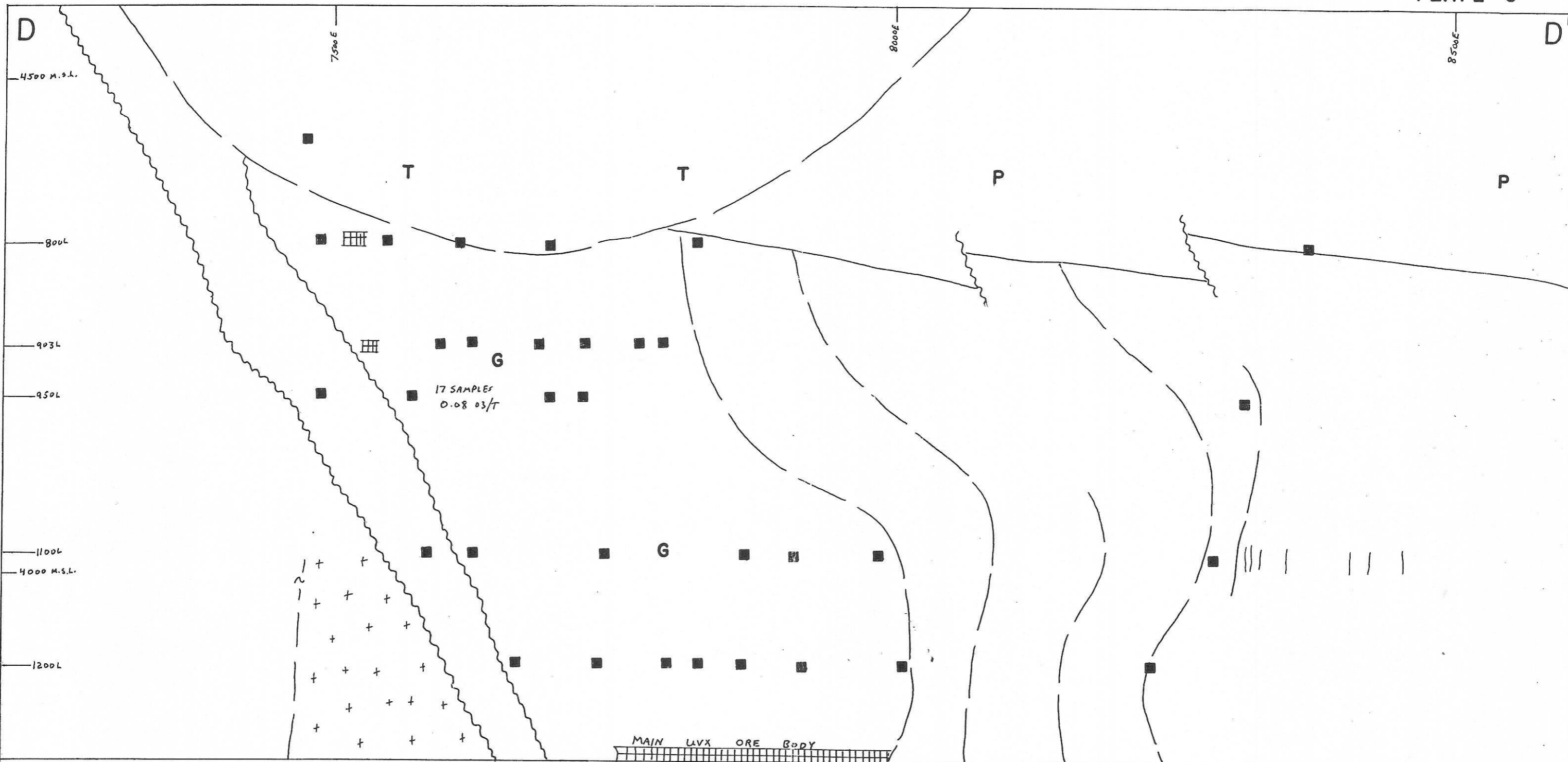
N. 62° E. CROSS SECTION DD' UVX MINE, JEROME, ARIZONA, LOOKING NORTHWEST AVAILABLE GOLD ASSAYS NOTED
