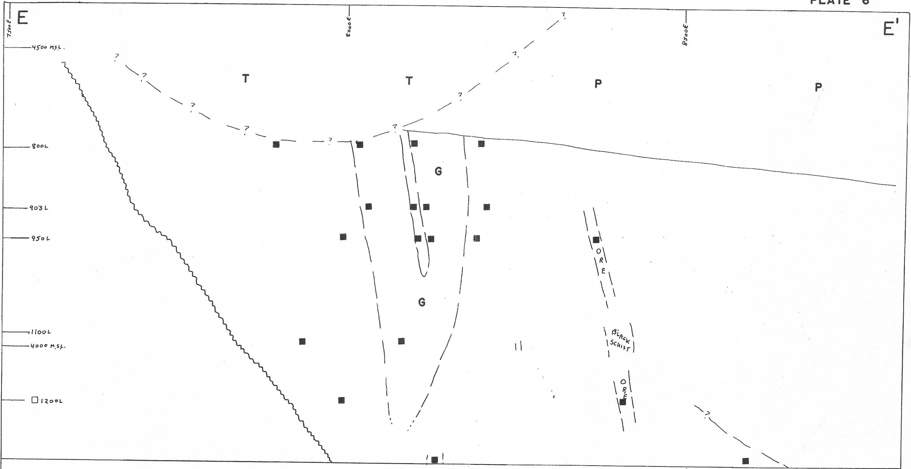
N. 62° E. CROSS SECTION EE' UVX MINE, JEROME, ARIZONA, LOOKING NORTHWEST AVAILABLE GOLD ASSAYS NOTED
