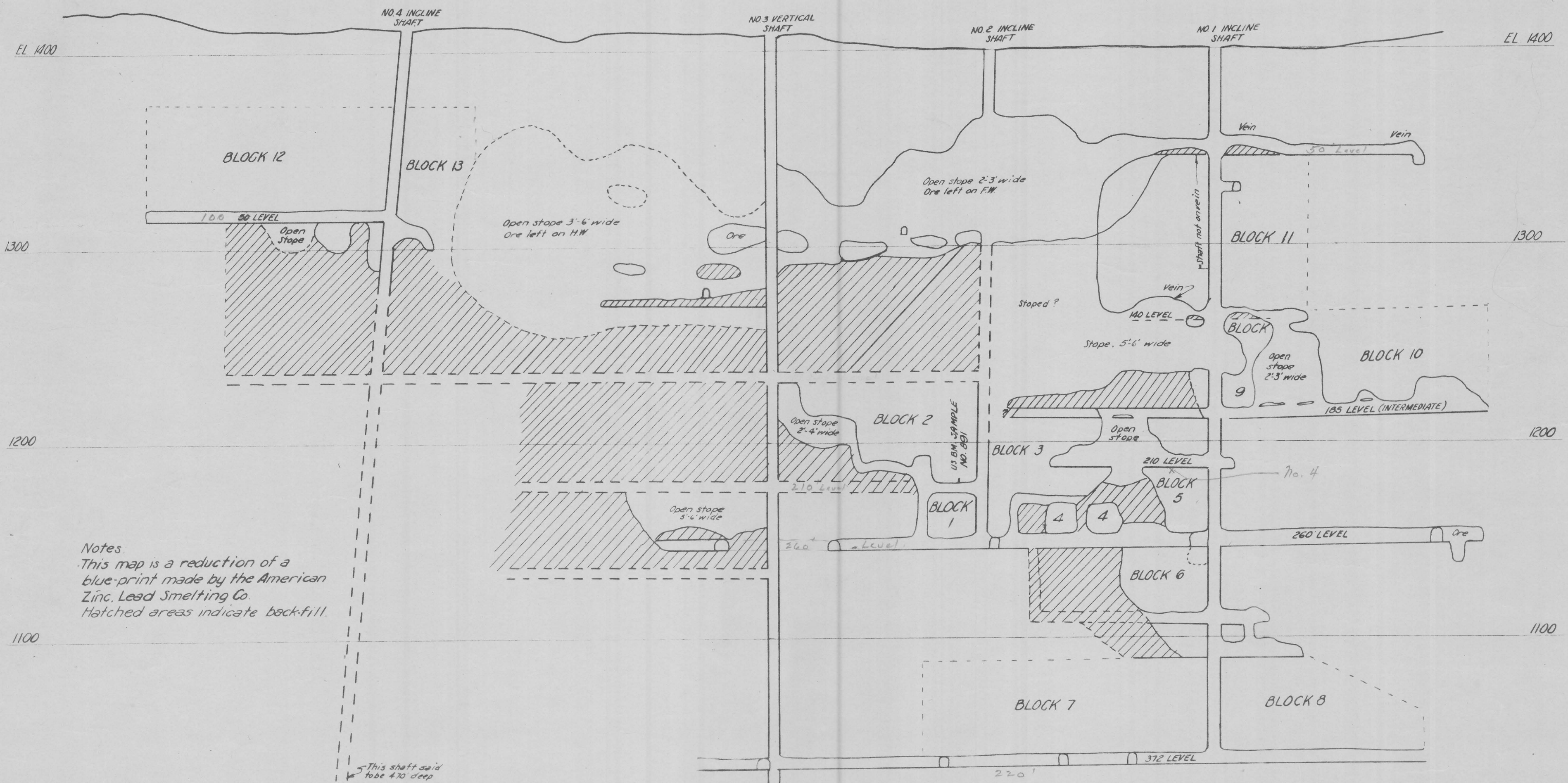
FIG 3 - LONGITUDINAL SECTION ON VEIN, RIALTO MINE, CASTLE DOME MINING DISTRICT, YUMA CO., ARIZ.
