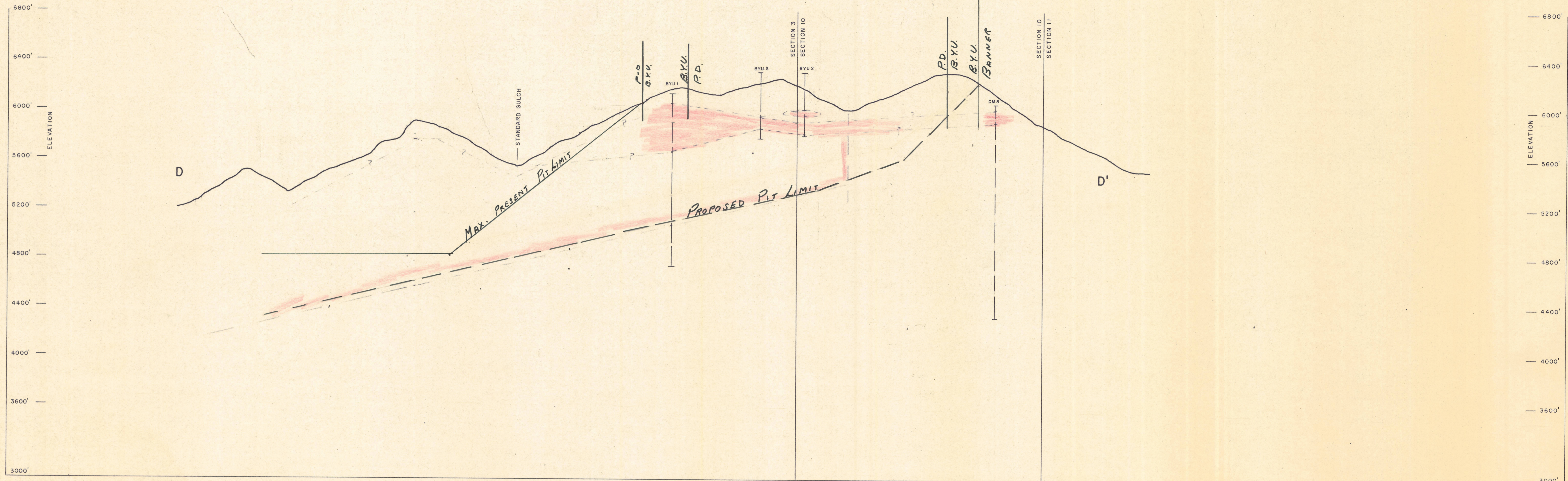
BOUNDARY FAULT SECTION D-D' LOOKING NORTH EAST SCALE 1"=400'
