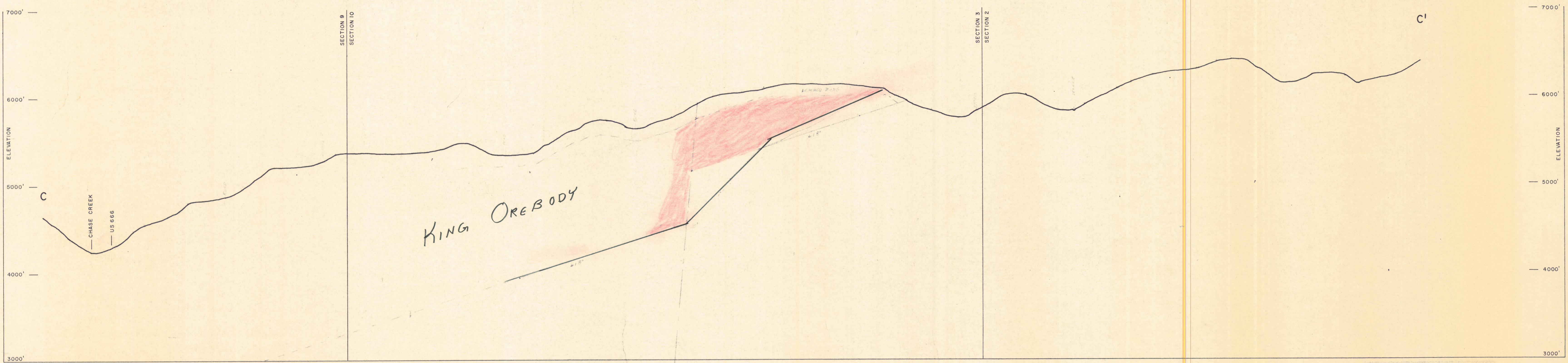
SECTION C-C' LOOKING NORTH WEST SCALE 1"=500'
