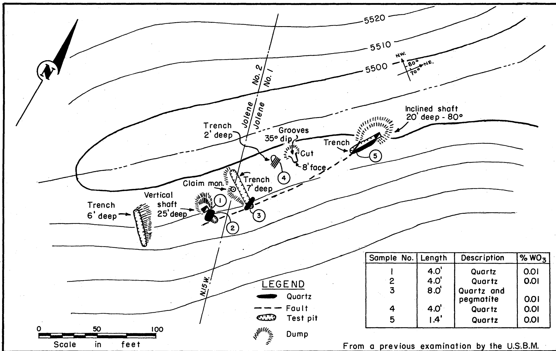
Figure 11. Transit-stadia survey - Jolene Tungsten, Gila County, Ariz.
